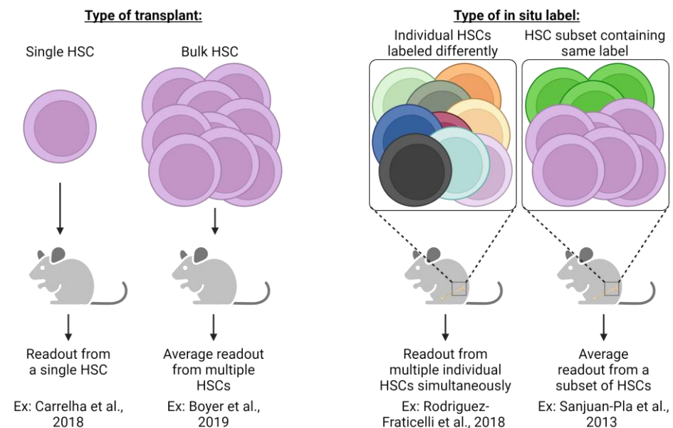
Figure 3. Different experimental strategies require unique interpretations. The experimental approach utilized in lineage tracing studies (transplantation or in situ labeling) necessitates specific interpretation of results and understanding of potential caveats. Single HSC transplants allow an assessment of cellular output from an individual HSC clone, yet readout may be underestimated due to the potential for relatively low-donor-derived chimerism that could be below the method of detection employed. Conversely, bulk HSC transplants significantly improve the detection of donor-derived cells, yet the output of individual HSCs is not possible to assess but is rather the average response of all HSCs transplanted. In situ label induction that uniquely labels each HSC clone allows for the simultaneous assessment of each clone yet may suffer from the same limitations as single-cell HSC transplants (i.e., underestimation of individual HSC contribution due to limits of detection). Similar to bulk HSC transplants, genetic labeling strategies label only a subset of heterogenic HSCs whose measured output is the average of all labeled cells. Both transplantation and in situ labeling also have the potential to skew resulting data and interpretation due to the cell surface phenotype or type of label induction employed. For example, fluorescent genetic reporters may be detectable in platelets, but genetic barcoding approaches are undetectable due to lack of genetic material. If only some heterogeneous HSC clones are assessed, then results can only be understood based on the phenotypic or transcriptomic profile used experimentally [20,68,70,80].
