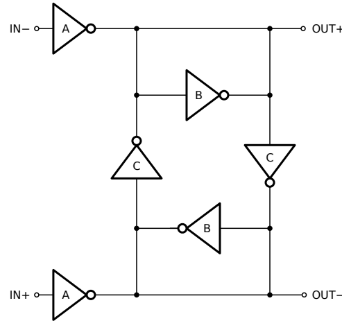
Figure 6. Nauta (N) OTA circuit diagram [2].
