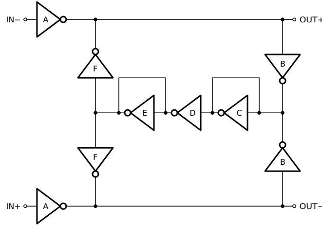
Figure 8. Mafredini (M) OTA circuit diagram [11].
