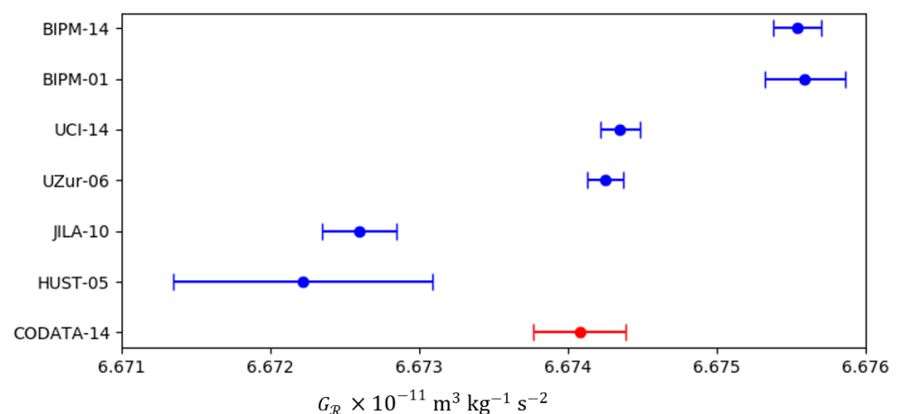
Figure 2. Six precision measurements of the G_{\mathcal{R}} values among those that were adopted in the CODATA 2014 recommended value.
