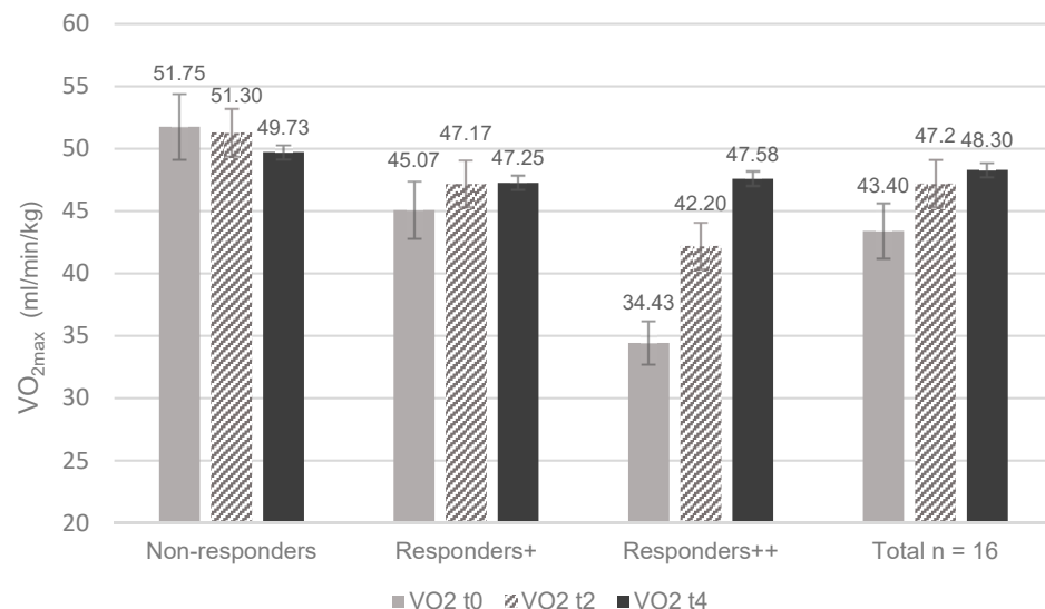
Figure 3. \text{VO}_2\text{max} (mL/min/kg) improvement (t0–t4) by category ("nonresponders", n = 6 , -14.3 – 1.0\% ; "responders+", n = 5 , 7.4 – 16.8\% ; "responders++", n = 5 , 23 – 62.5\% ) and for the total sample. Values are shown as mean and 95% CI.
