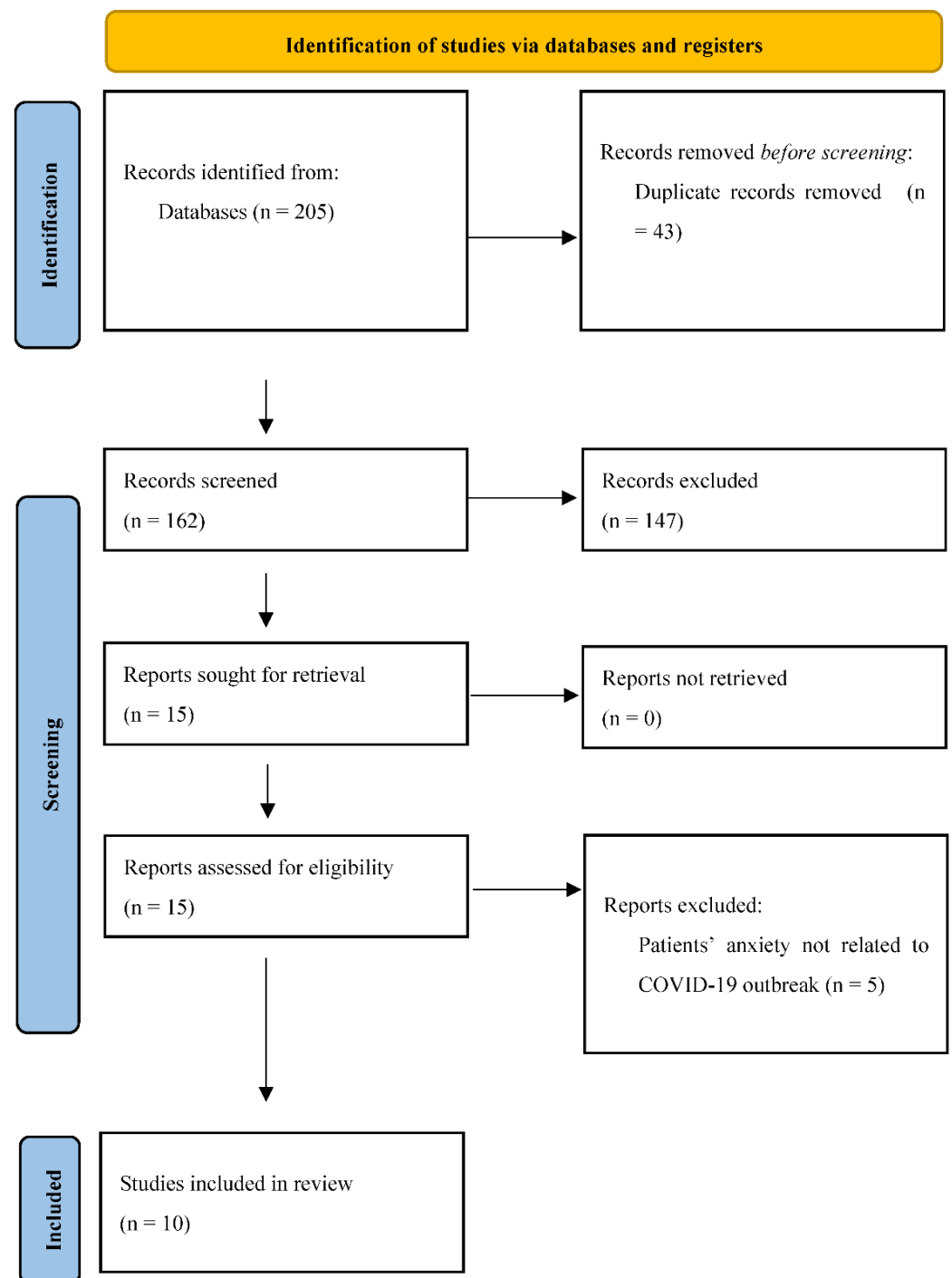
Figure 1. PRISMA Flow-chart.
