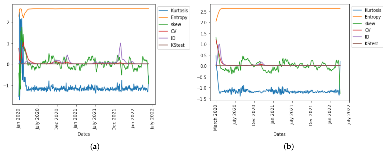
Figure 12. Various statistical predictor indicators for the COVID-19 pandemic in the UK for (a) daily new cases and (b) daily deaths.
