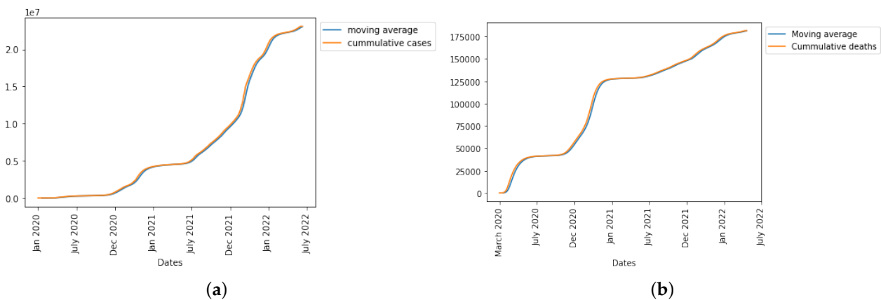
Figure 2. (a) Cumulative cases and (b) cumulative deaths with their moving average (in blue) as at July 2022.
