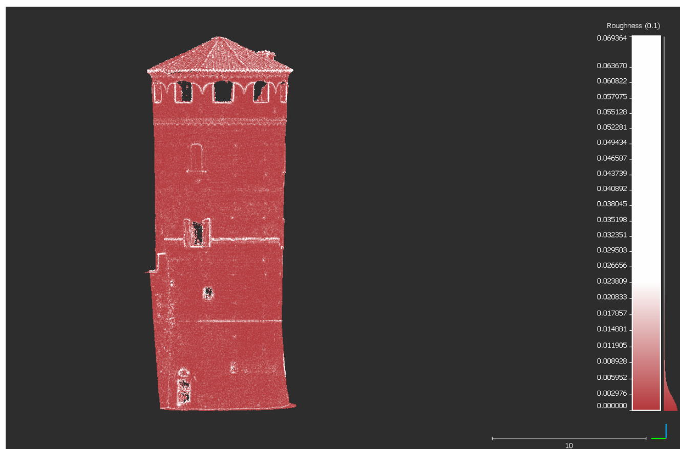
Figure 28. Roughness analysis of the photogrammetric data: RMSe 0.006 m; standard deviation 0.005 m. White points are related to roughness and noise record.
