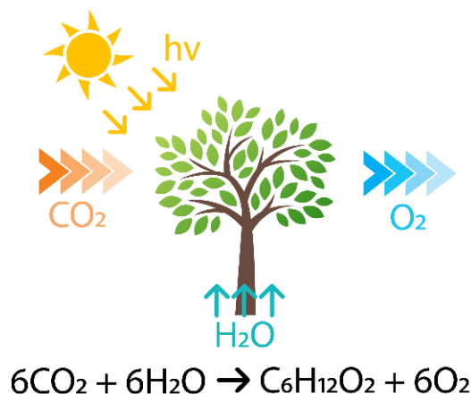
Figure 2. Photosynthesis reaction.
