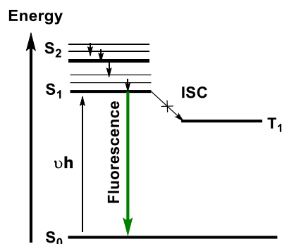
Figure 15. Simplified Jablonski diagram for fluorescence.
