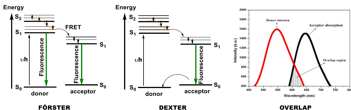
Scheme 1. Quenching mechanism of fluorescence using a Jablonski diagram. Forster (left) [39], Dexter (middle), and the right overlap between the emission and absorption (right). Adapted with permission from Ref [40], Copyright 2011, Elsevier.
