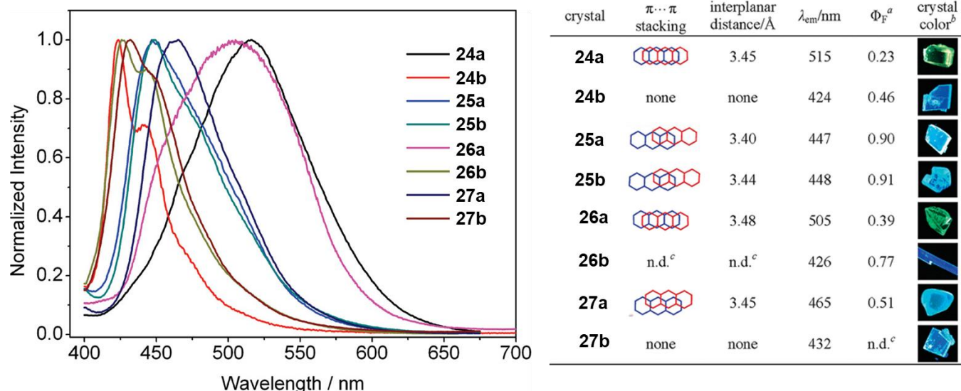
Figure 30. Solid-state emission (left), crystal packing of compounds 24–27 and their photophysical properties (right). Adapted with permission from Ref. [81]. Copyright 2009, American Chemical Society.
