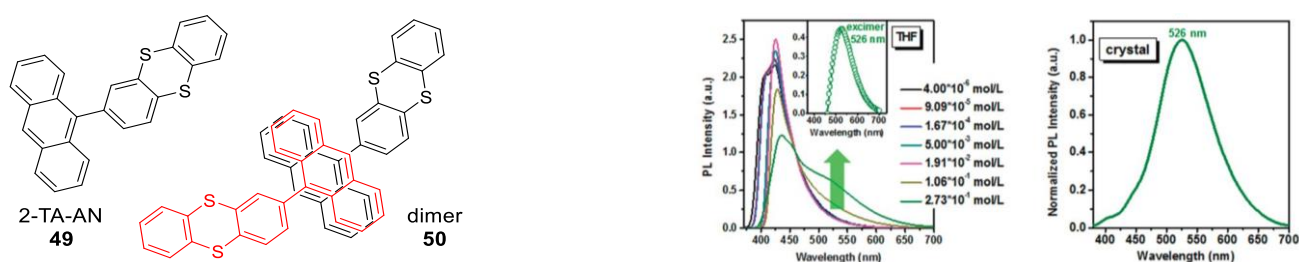
Figure 47. PL spectra recorded for 2-TA-AN in THF solutions with increasing concentration and in crystal form. Molecular structure of 2-TA-AN in solution and the intermolecular packing. Reprinted with permission from Ref. [109]. Copyright 2018, Royal Society of Chemistry.
