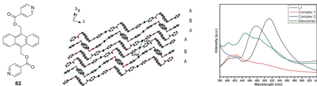
Figure 67. Chemical structure of L-82 ( left ), packing of the coordination polymer chains ( center ) and emission spectra of 82 and complex ( right ), (excitation wave length is 344 nm). Adapted with permission from Ref. [107]. Copyright 2013, The Royal Society of Chemistry.
