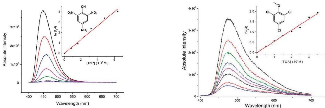
Figure 65. Fluorescence sensing of picric acid (TNP) ( left ) and 2,4,6-trichloroanisole (TCA) ( right ) by 88d in MeCN. Adapted with permission from Ref. [23]. Copyright 2019, American Chemical Society.
