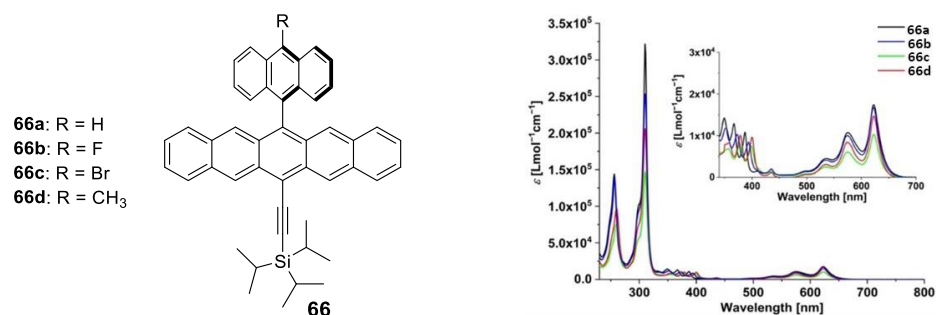
Figure 56. Structure (left), UV–VIS absorption spectra of 66a–d (measured in CH 2 region of 225–800 nm and expansion from 340–700 nm (right)). Reprinted with permission from Ref. [130]. Copyright 2020, Wiley-VCH Verlag GmbH & Co.
