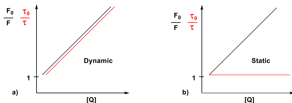
Figure 16. Stern–Volmer graph for dynamic (a) and static (b) quenching.
