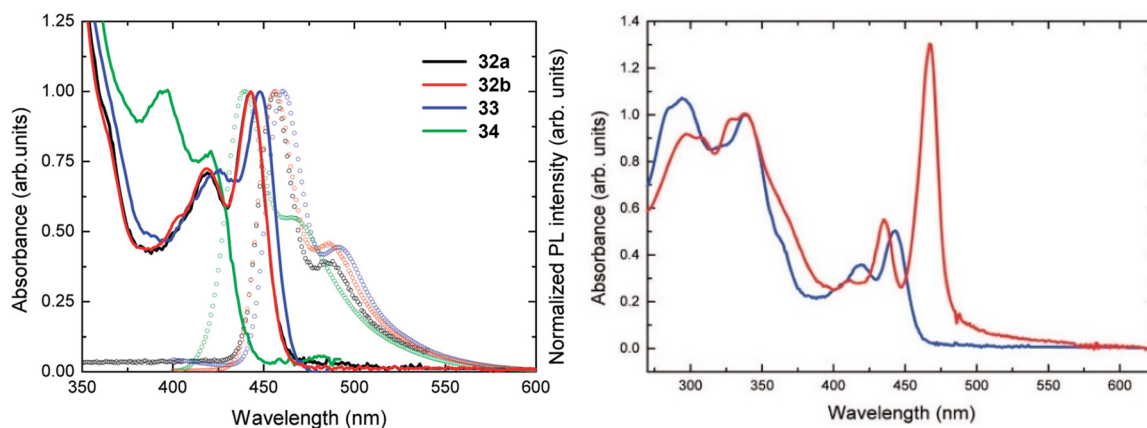
Figure 38. Normalized absorbance (solid lines) and emission (dotted lines) spectra of 32a, 32b, 33, and 34 in chloroform (left) and absorption spectra of 32a, solution (blue) vs. film (red) (right). Reprinted with permission from Ref. [94]. Copyright 2009, American Chemistry Society.
