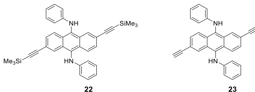
Figure 26. Structures of 22 and 23 anthracene derivatives.
