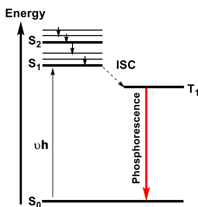
Figure 17. Simplified Jablonski diagram for phosphorescence.
