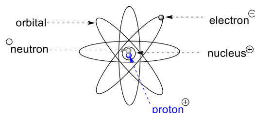
Figure 5. Atomic structure.
