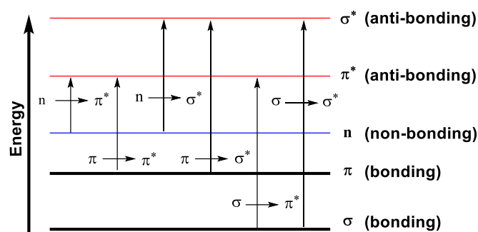
Figure 7. Most common electronic transitions ( n , \pi , \sigma ).
