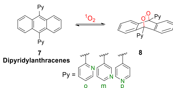
Scheme 4. Oxygenation of dipyriddylanthracenes and reversion of the aromatic endoperoxides EPOs. Adapted with permission from Ref. [64]. Copyright 2017, American Chemical Society.
