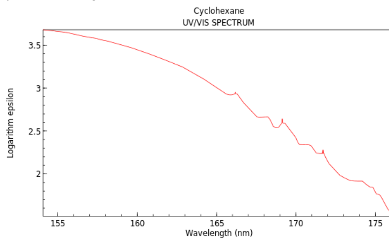
Figure 11. UV-VIS spectrum of cyclohexane. Reprinted with permission from Ref. [8]. Copyright 2019, Elsevier.
