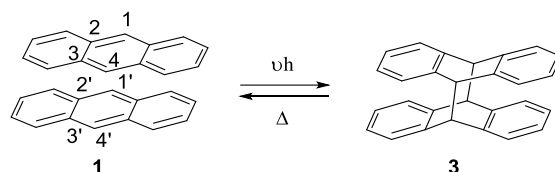
Figure 18. Anthracene photodimerization. Adapted with permission from Ref. [65]. Copyright 1867, Verlag GmbH & Co. KGaA, Weinheim.
