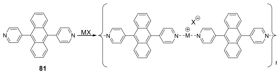
Figure 66. 1D coordination polymer of 81 in the presence of the metal ( \text{M} = \text{Ag}^{\text{I}} , \text{Zn}^{\text{II}} , \text{Cd}^{\text{II}} , or \text{Hg}^{\text{II}} ) in 1:1 ratio \text{M} = \text{Ag}^{\text{I}} , \text{Zn}^{\text{II}} , \text{Cd}^{\text{II}} , or \text{Hg}^{\text{II}} ; \text{X} = \text{NO}_3^- , \text{CF}_3\text{COO}^- , \text{CH}_3\text{COO}^- , \text{Cl}^- , \text{BF}_4^- , \text{ClO}_4^- . Adapted with permission from Ref. [141]. Copyright 2009, WILEY-VCH Verlag GmbH & Co. KGaA.
