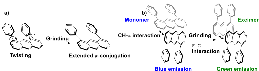
Scheme 6. Possible mechanism for the mechanofluorochromism of the 1,8-diphenylanthracene derivatives, (a) twisting of phenyl groups, and (b) excimer formation after grinding. Reprinted permission from Ref. [72]. Copyright 2021, Elsevier B.V.
