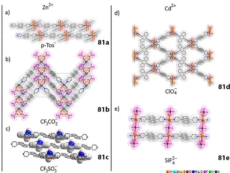
Figure 64. 1D (a–c) and 2D (d,e) coordination polymers obtained using ligand 81 with different metals ( \text{Zn}^{\text{II}} , or \text{Cd}^{\text{II}} ) and anions ( p\text{-Tos}^- , \text{CF}_3\text{CO}_2^- , \text{CF}_3\text{SO}_3^- , \text{ClO}_4^- , \text{SiF}_6^{2-} ). Adapted with permission from Ref. [23]. Copyright 2019, American Chemical Society.
