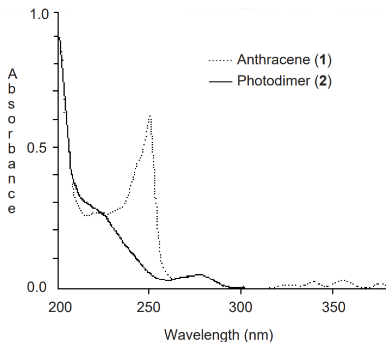
Figure 19. Comparative UV spectra of 1 ( 4 \times 10^{-6} M) and 3 ( 5 \times 10^{-5} M) as solutions in \text{CH}_3\text{CN} . Reprinted with permission from Ref. [66]. Copyright 1955, American Chemical Society.
