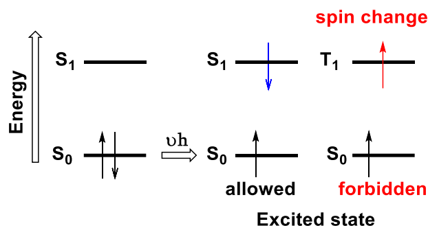
Figure 13. Spin selection rule \Delta S = 0 .
