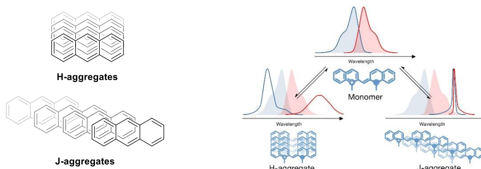
Figure 31. Possible H- and J-aggregate of anthracene ( left ) and schematic representation of the changes in absorption (blue) and fluorescence (red) for cyanine dye monomers ( right ). Reprinted/adapted with permission from Ref. [86]. Copyright 2017, iop Publishing Ltd.
