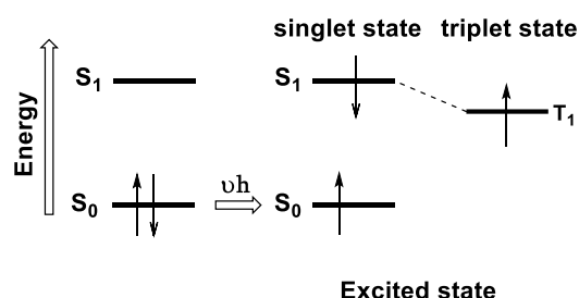
Figure 8. Singlet and triplet excited state.
