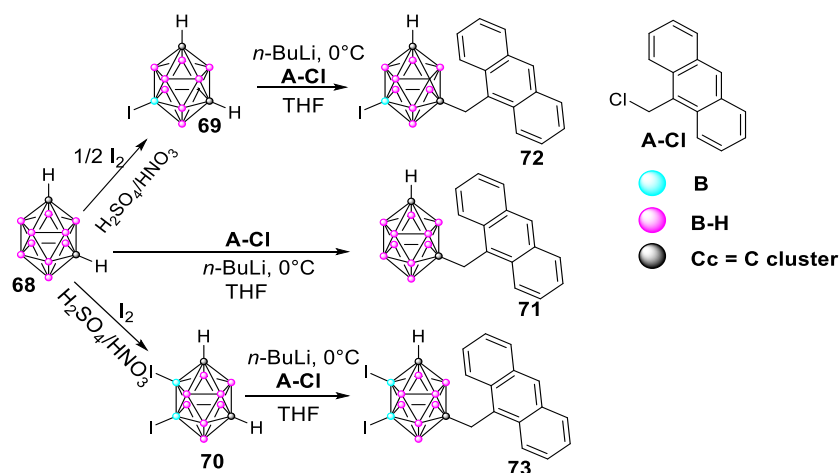
Scheme 11. Synthesis and characterization of anthracenyl-monosubstituted m-carborane derivatives 71 , 72 , and 73 . Reprinted with permission from Ref. [132]. Copyright 2019, The Royal Society of Chemistry.
