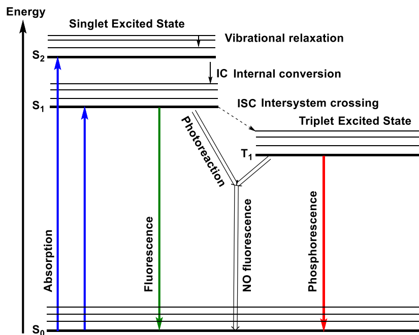
Figure 14. Jablonski diagram.
