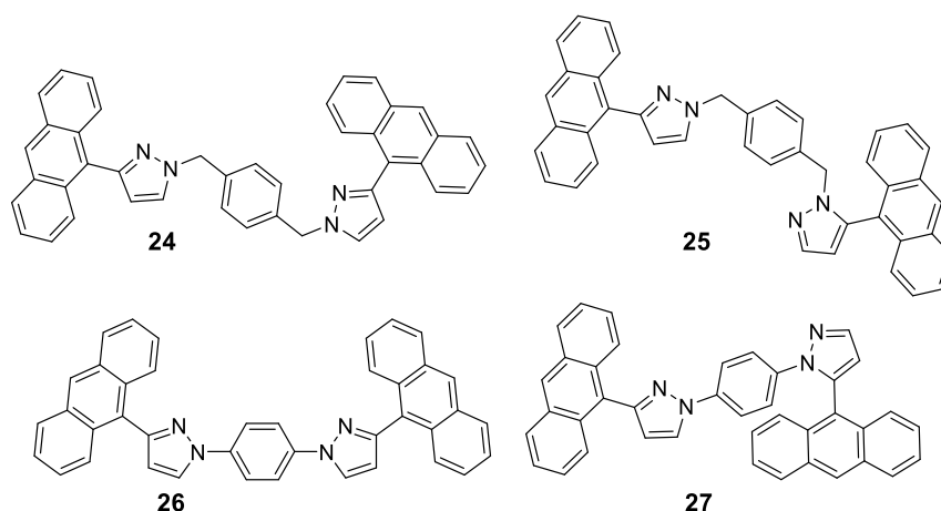
Figure 28. Anthracene derivatives 24–27 structures. Adapted with permission from Ref. [81]. Copyright 2009, American Chemical Society.
