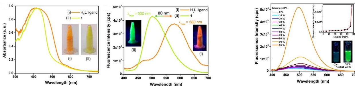
Figure 69. ( Left ) Solid-state absorption and ( middle ) emission spectra of Cp and 83 ligand at room temperature. ( Right ) Change in the fluorescence emission spectra of 83 ligand (50 μM) with a change of hexane vol% in ethanol. Adapted with permission from Ref. [147]. Copyright 2017, American Chemistry Society.
