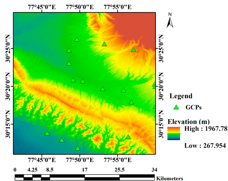
Figure 4. GCPs collected using DGPS survey are overlaid on simulated MLP DEM product.
