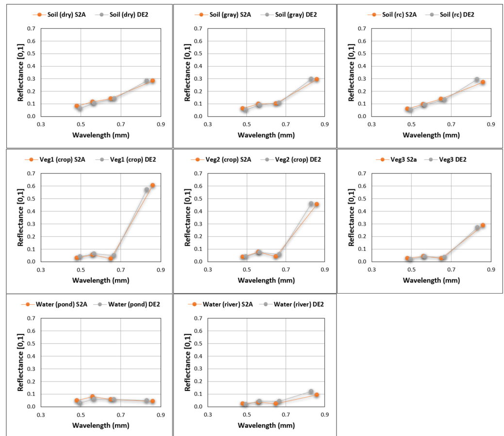
Figure 4. Vegetation, soil and water spectral profiles comparison between DE2/SE2 bands.
