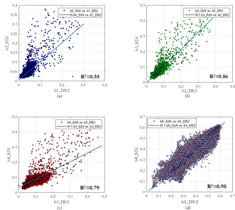
Figure 3. Regression analysis (Vertical/Horizontal axis units [0,1] a.u.). (a) Blue bands, Band 2 S2A vs. Band 1 DE2; (b) Green bands, Band 3 S2A vs. Band 2 DE2; (c) Red bands, Band 4 S2A vs. Band 3 DE2; (d) NIR bands, Band 8 S2A vs. Band 4 DE2.
