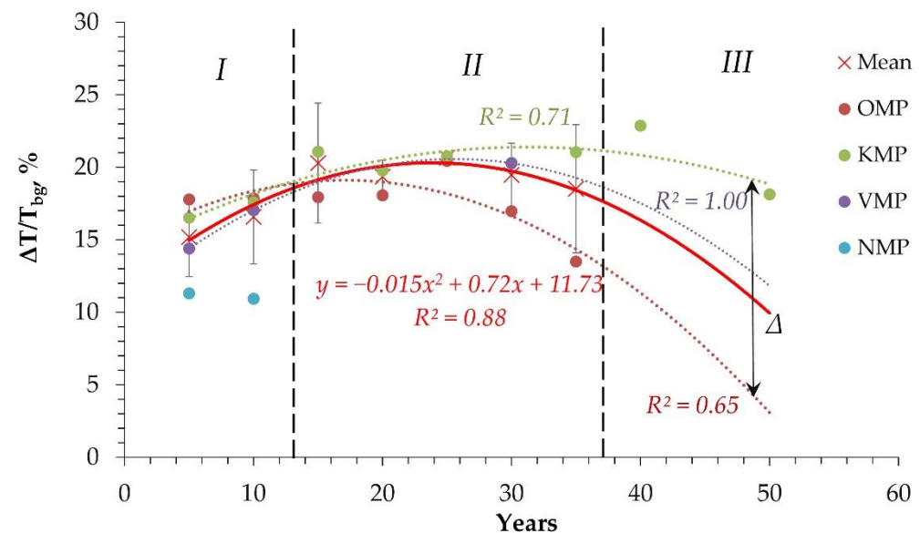
Figure 3. Thermal anomalies in disturbed areas of selected technogenic plots: (×) average for all areas. (OMP) Olimpiada, (KMP) Kuranakh, (VMP) Verninskoye, (NMP) Natalka. Initial stage of technogenic impact (I), the stage of technogenic activity (II), and post-technogenic recovery stage (III) have been marked out.
