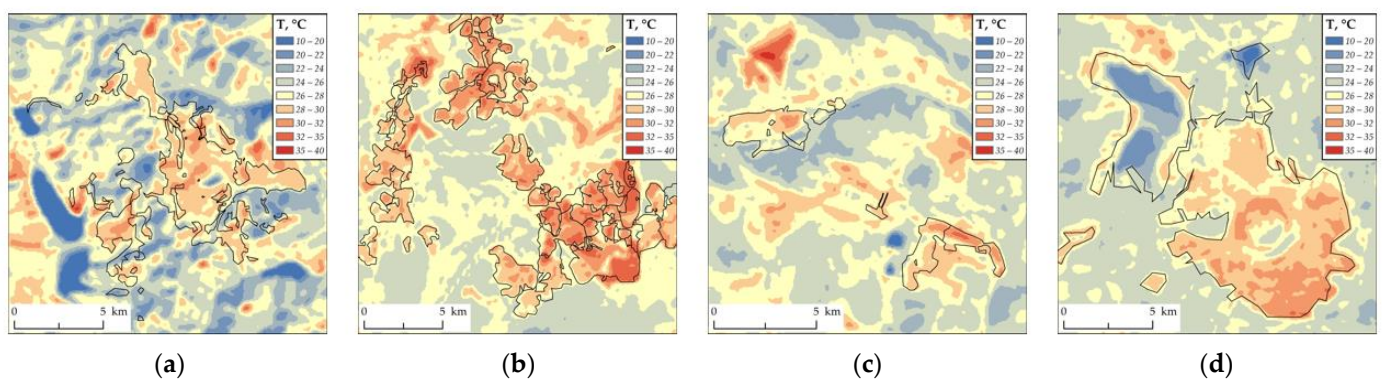
Figure 2. Temperature field for technogenic plots of (a) NMP (Magadan Region), (b) VMP (Irkutsk Region), (c) KMP (Republic of Sakha (Yakutia)), and (d) OMP (Krasnoyarsk Region).
