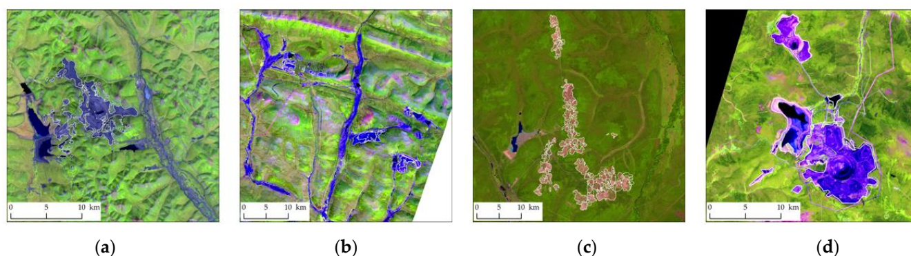
Figure 1. Area of disturbances from Landsat-8/OLI images of 2015–2020 for technogenic plots of (a) NMP (Magadan Region), (b) VMP (Irkutsk Region), (c) KMP (Republic of Sakha (Yakutia)), and (d) OMP (Krasnoyarsk Region).
