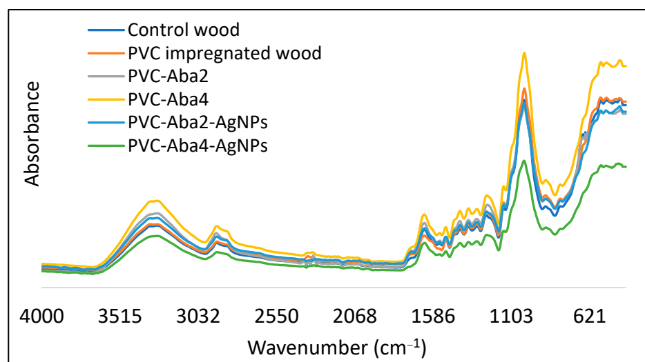
Figure 3. FTIR-ATR spectrum of the wood and impregnated wood.
