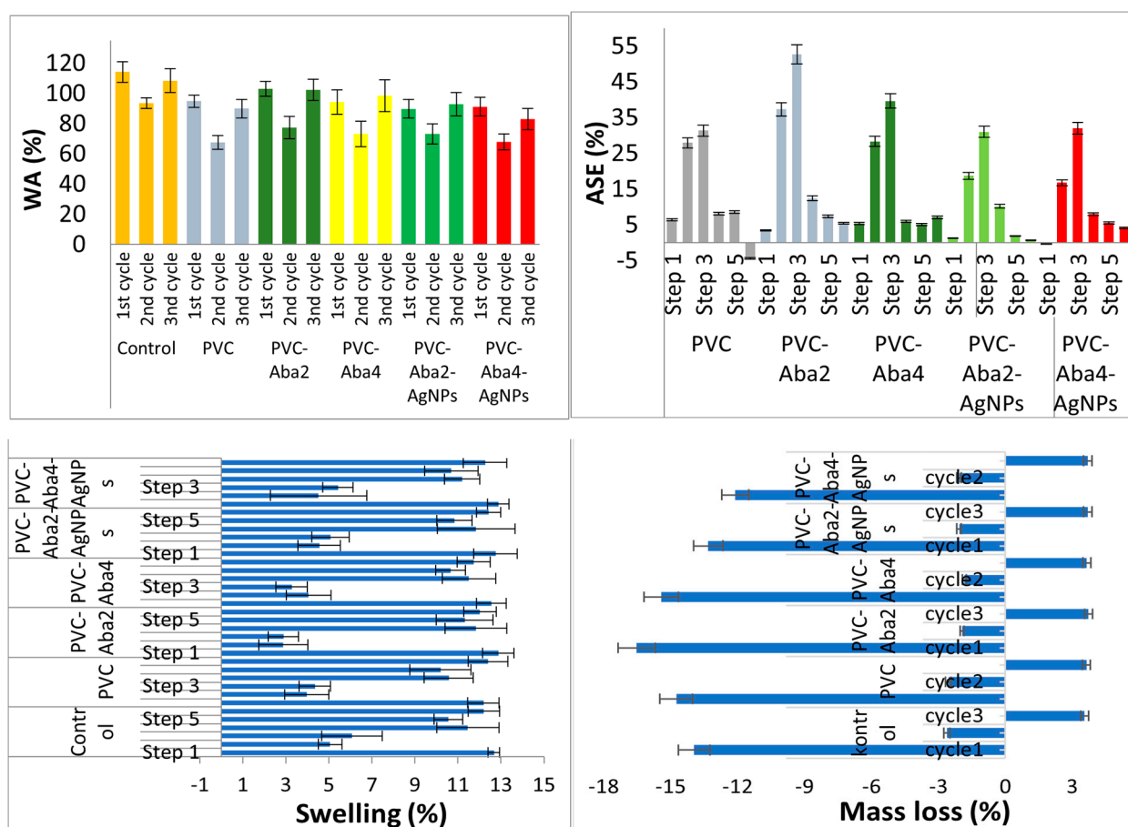
Figure 1. ASE (Average anti-swelling efficiency values %), swelling values, mass loss values by leaching, and water uptake values of untreated and modified samples.
