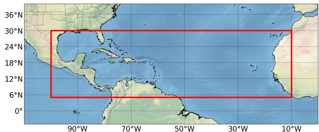
Figure 1. The red box (5–30° N in latitude and 10–100° W in longitude) delimits the area in which the annual mean Sea Surface Temperature and the Maximum Potential Intensity were computed.
