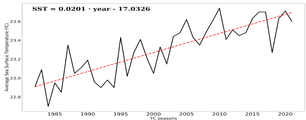
Figure 2. Annual averaged SST in the red box showed in Figure 1. The red dashed line denotes the trend line statically significant at 95%.
