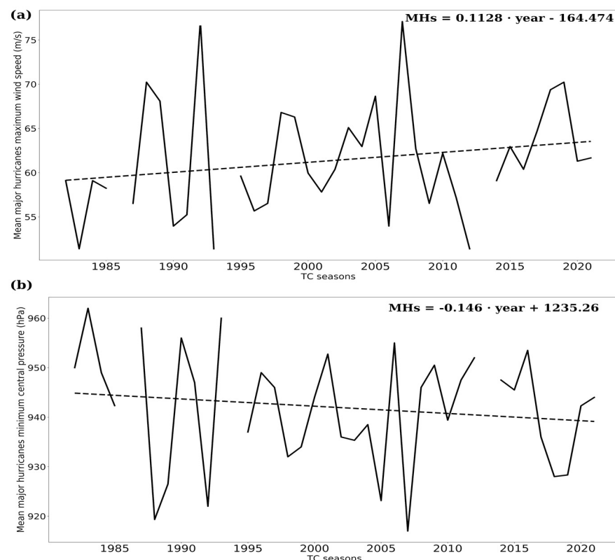
Figure 3. Annual averaged of (a) maximum wind speed and (b) minimum central pressure for the major hurricanes, based on the HURDAT2 database. The black dashed line represents the linear trend ( p > 0.05 ). The discontinuities in the black solid lines denotes a TC season without major hurricanes.
