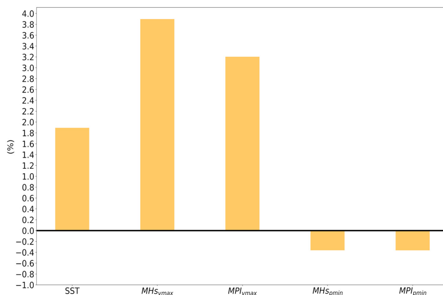
Figure 5. Changes (in percentage) of the mean Sea Surface Temperature, major hurricane intensity and maximum potential intensity in the period 2002–2021 in relation to the period 1982–2001.
