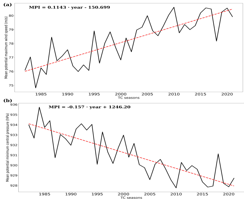
Figure 4. Annual averaged of (a) potential maximum wind speed and (b) potential minimum central pressure based on the HuMPI model outputs. The red dashed line represents the linear trend statistically significant at 95%.
