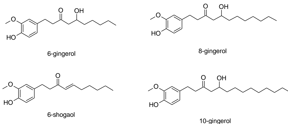
Figure 3. The structures of 6-gingerol, 6-shogaol, 8-gingerol and 10-gingerol.
