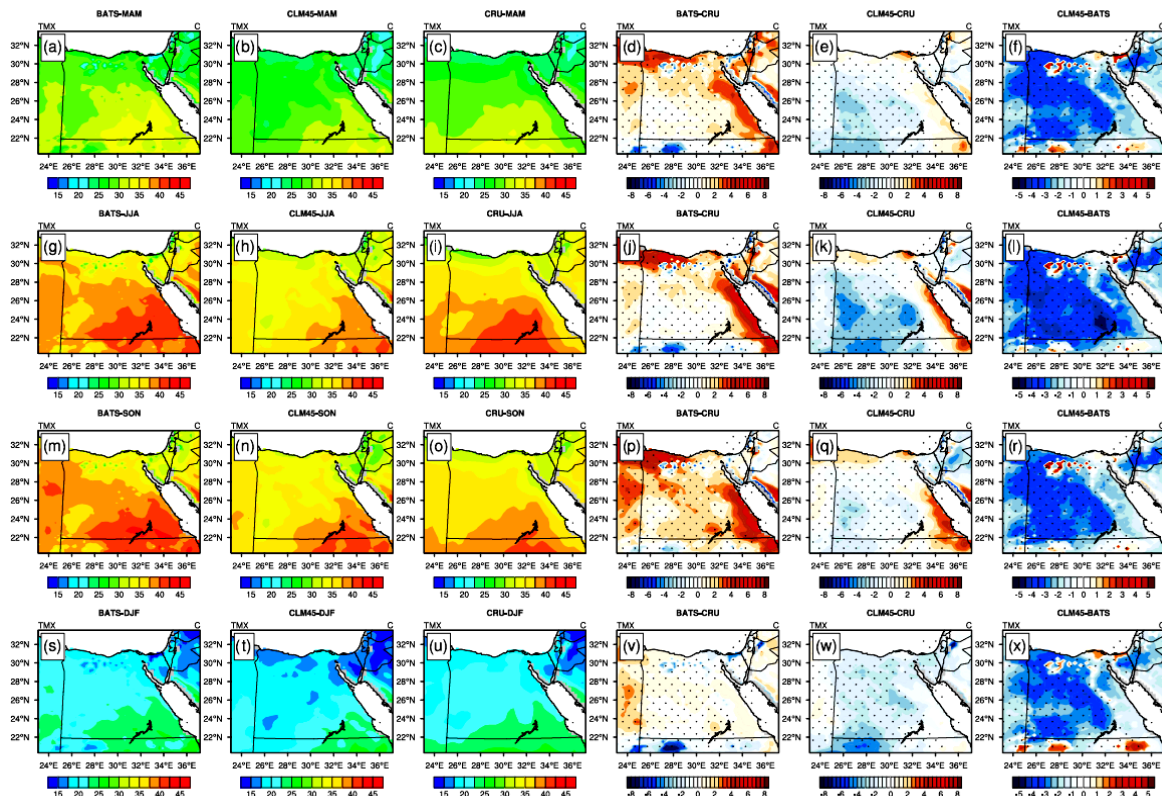
Figure 6. The figure shows the simulated daily maximum air temperature over the period of 2001–2010 (TMX; in °C) for the seasons: MAM in the first row (a–f); JJA in the second (g–l); SON in the third (m–r); and DJF in the fourth (s–x). For each row, BATS is on the left, followed by CLM45. CRU is the third from left, followed by BATS minus CRU, CLM45 minus CRU and the difference between CLM45 and BATS. Significant difference/bias is indicated with black dots using Student t -test with alpha equal to 5%.
