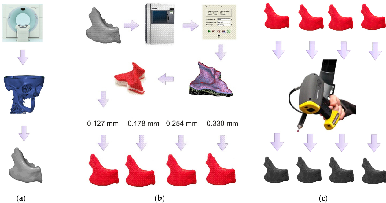
Figure 1. The procedure applied in the research process: (a) the reconstruction process of the zygomatic bone geometry; (b) the manufacturing process using the FDM technology; (c) the measuring process using a measuring arm and laser head.
