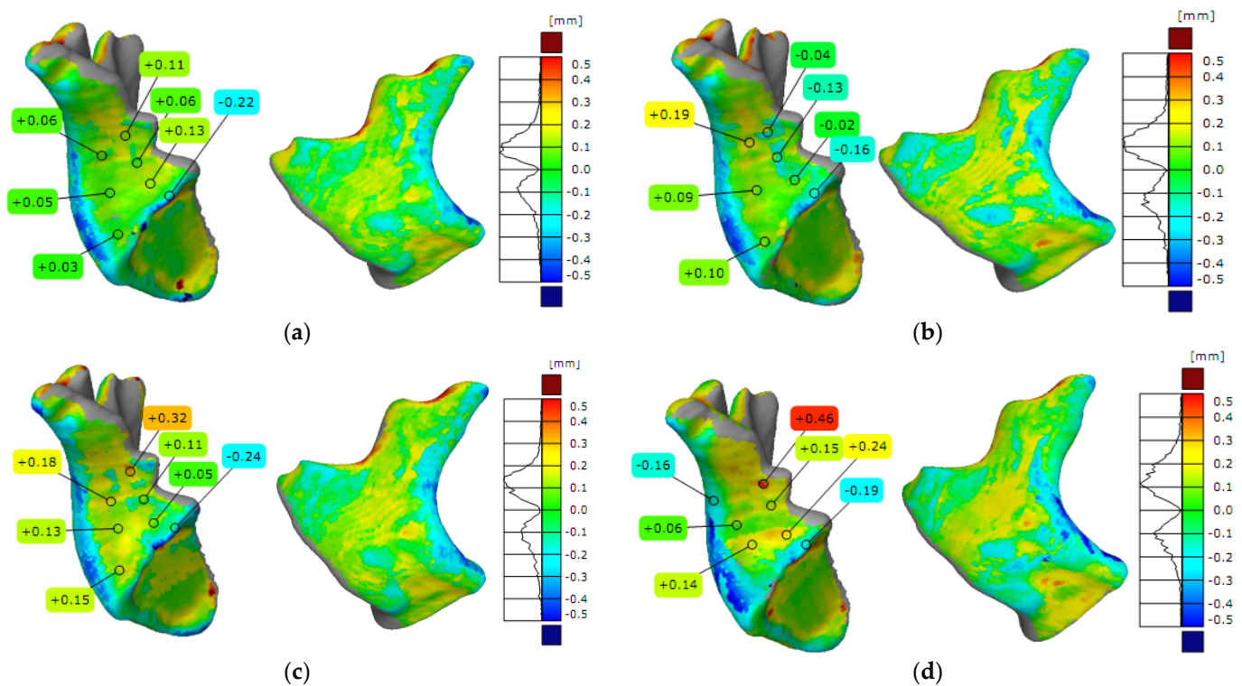
Figure 2. The results of the accuracy of manufacturing zygomatic bone geometry: (a) model manufactured with an applied layer thickness of 0.127 mm; (b) model manufactured with an applied layer thickness of 0.178 mm; (c) model manufactured with an applied layer thickness of 0.254 mm; (d) model manufactured with an applied layer thickness 0.330 mm.
