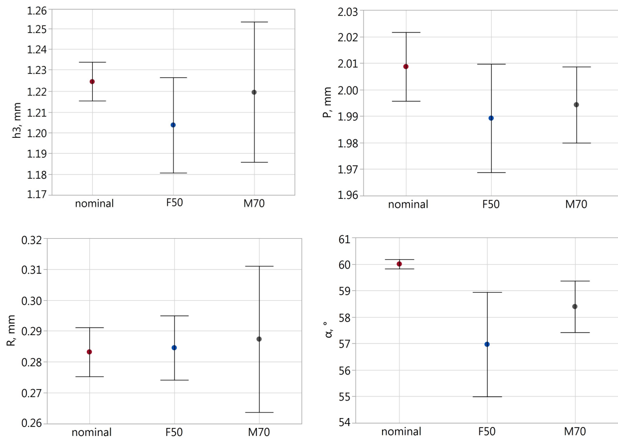
Figure 1. Values of thread height h_3 , pitch P , root radius R and thread angle \alpha measured directly and using F50 and M70 replicas.
