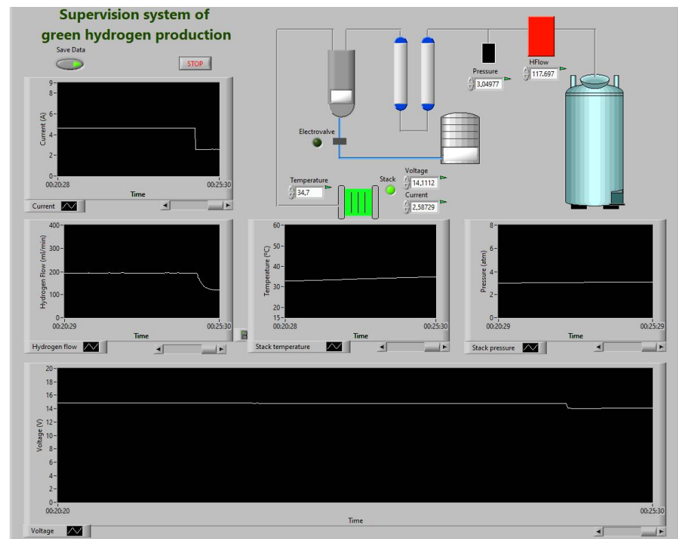
Figure 3. LabVIEW graphical interface to supervise green hydrogen production.
