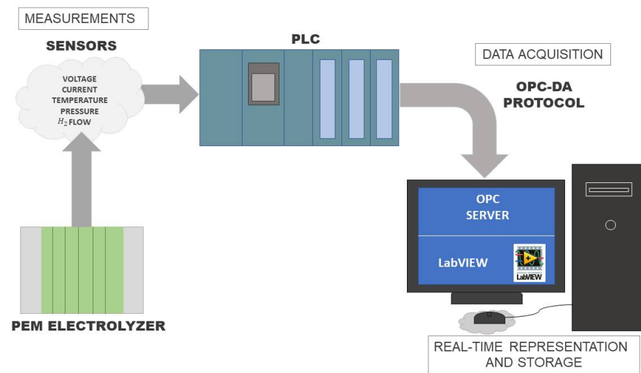
Figure 2. Supervision system and interaction between components.
