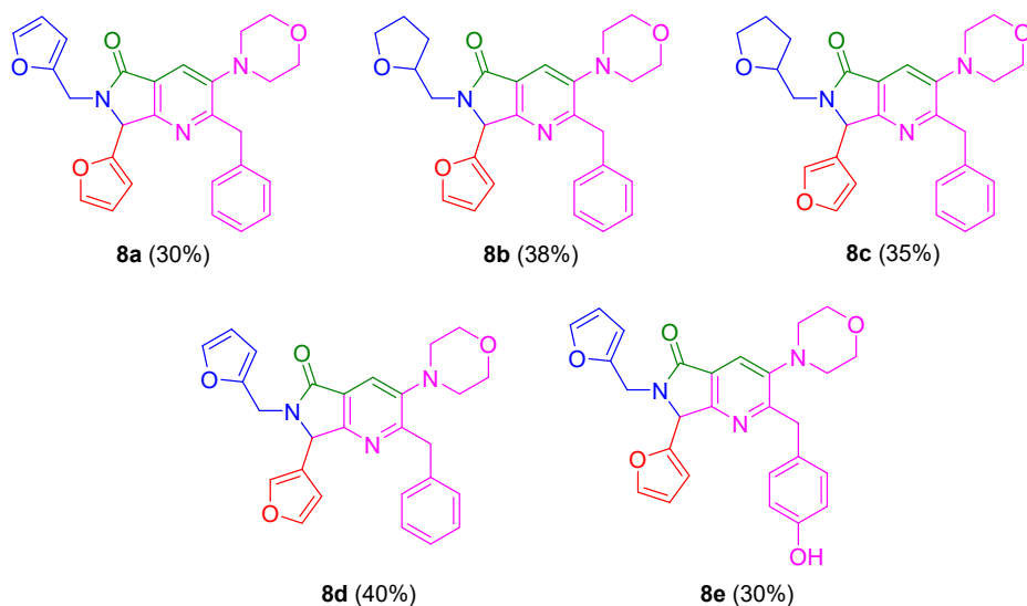
Scheme 2. Synthesis of pyrrolo[3,4-b]pyridin-5-ones via a cascade process (Ugi-Zhu/ aza -Diels-Alder/ N -acylation/aromatization).
