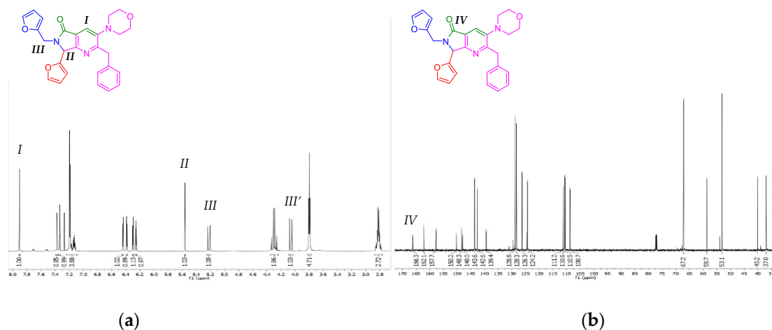
Figure 2. (a) ^1H NMR spectrum of the compound 1a , (b) ^{13}C NMR spectrum of the compound 8a .
