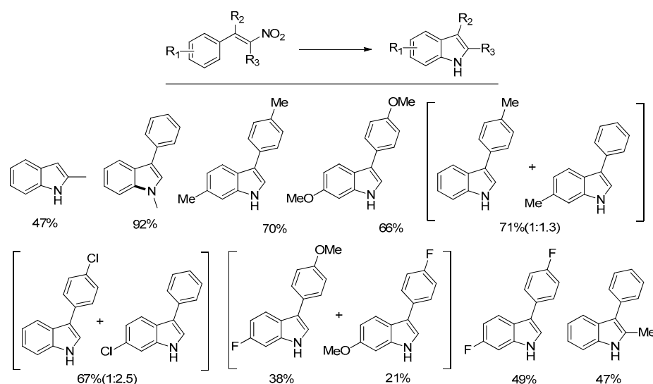
Figure 2. Synthesis of indoles from \beta -nitrostyrenes. Experimental conditions: 0.54 mmol nitrostyrene, 1 mol% \text{PdCl}_2(\text{CH}_3\text{CN})_2 , 5 mol% Phen, 260 \mu\text{L} \text{PhOC(O)H} , 120 \mu\text{L} \text{Et}_3\text{N} , in 10 mL \text{CH}_3\text{CN} , at 140 ^\circ\text{C} for 4 h.
