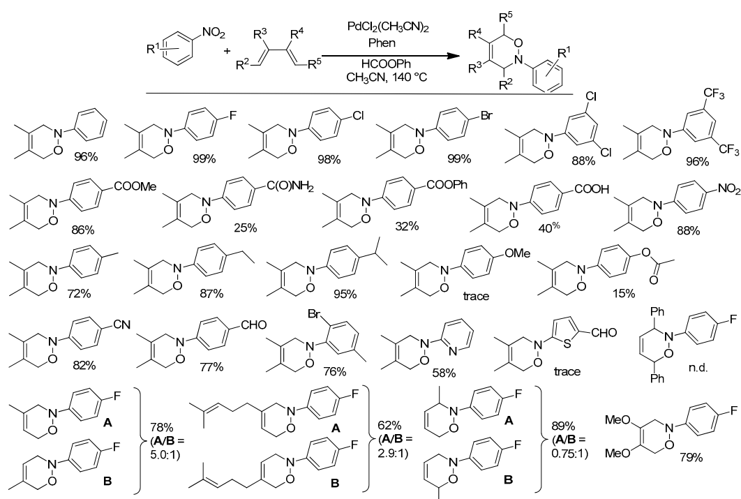
Figure 3. Synthesis of oxazines from nitroarenes and conjugated dienes. Experimental conditions: nitroarene 0.54 mmol, Pd(CH 3 CN) 2 Cl 2 1 mol%, Phen 2.5 mol%, diene 4 equiv, HCOOPh 2.2 mmol, Et 3 N 0.27 mmol, in 10 mL CH 3 CN, at 140 °C for 4 h.
