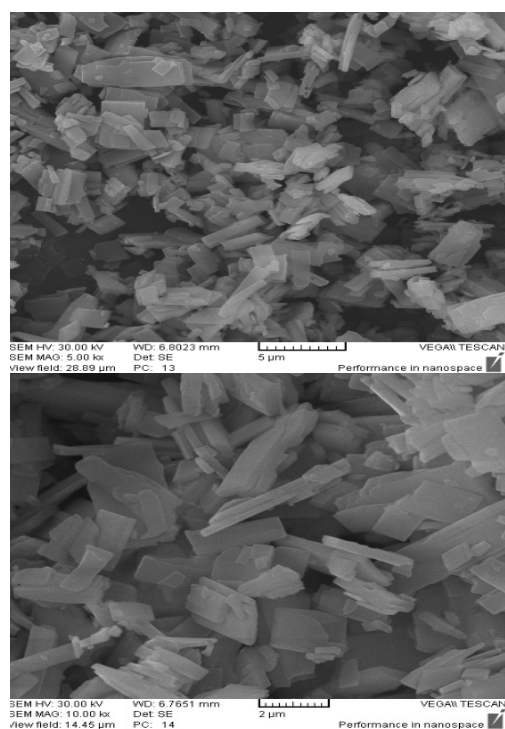
Figure 3. SEM of [\text{Ba}(\text{H}_2\text{btec})\cdot\text{H}_2\text{O}]_n .
