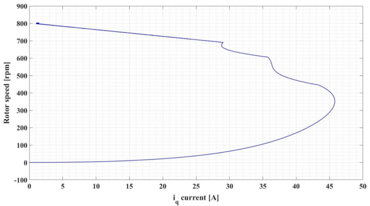
Figure 30. Image of the phase plan for PMSM variable structure with switching signal type 2: rotor speed versus i_q current ( \omega_{ref} = 800 rpm).
