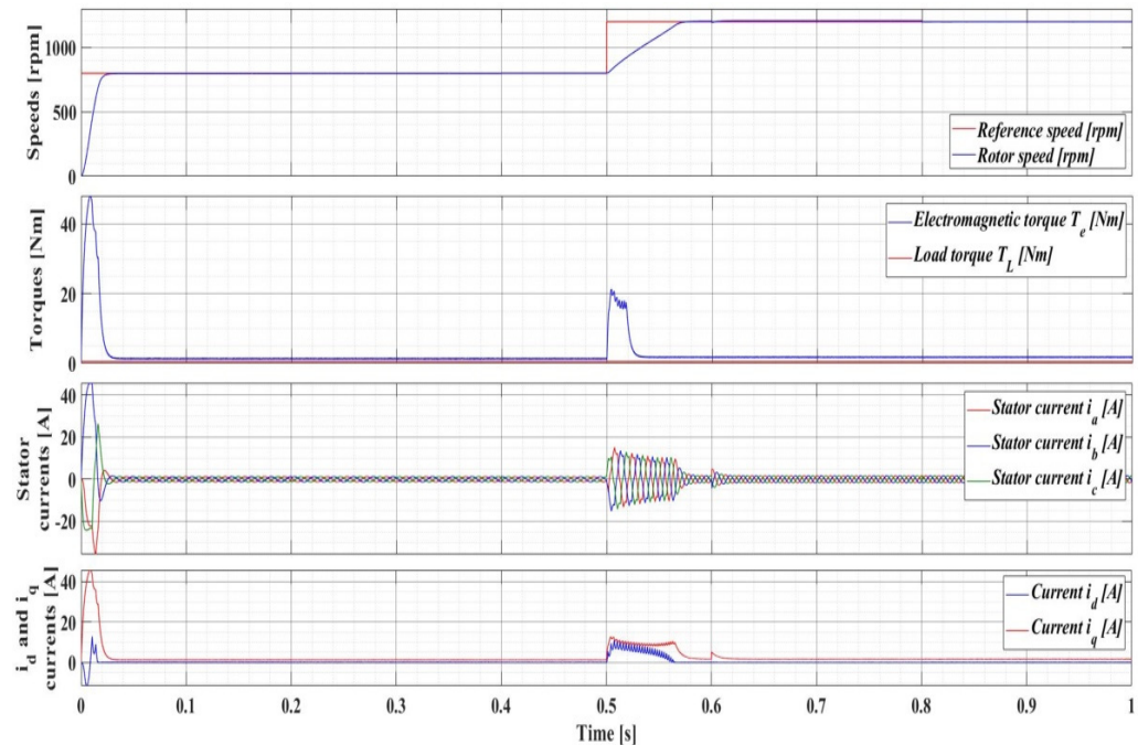
Figure 25. Time evolution for PMSM control system based on FOC-type strategy for PMSM with variable structure and switching signal type 2, \omega_{ref} = [800, 1200] rpm, and T_L = 0.5 Nm.
