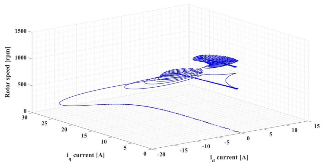
Figure 19. Image of the state space for PMSM variable structure with switching signal type 1: rotor speed versus i_q current versus i_d current ( \omega_{ref} = [800, 1200] rpm).
