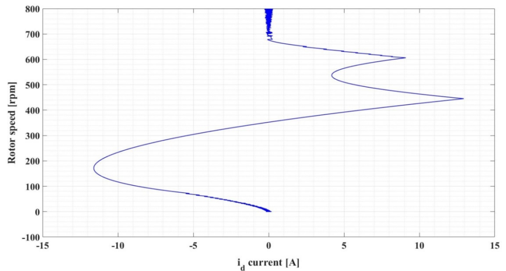
Figure 5. Image of the phase plan: rotor speed versus i_d current.
