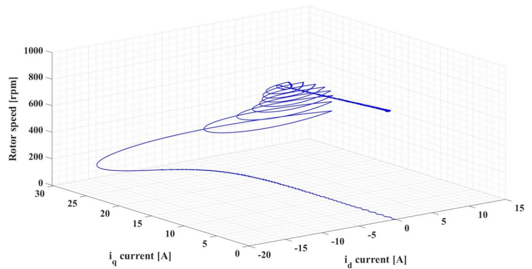
Figure 18. Image of the state space for PMSM variable structure with switching signal type 1: rotor speed versus i_q current versus i_d current ( \omega_{ref} = 800 rpm).
