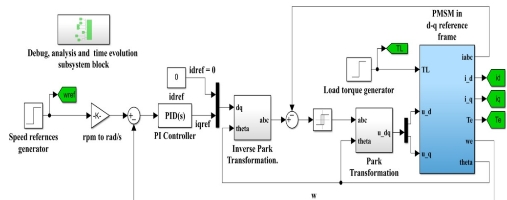
Figure 2. Simulink implementation for PMSM control system based on FOC-type strategy.
