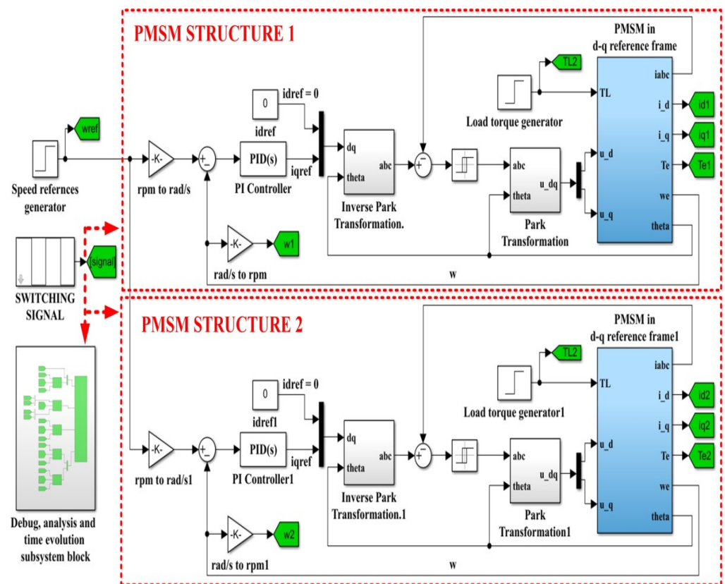
Figure 10. Simulink implementation for PMSM control system based on FOC-type strategy for PMSM variable structure with switching signal type 1.
