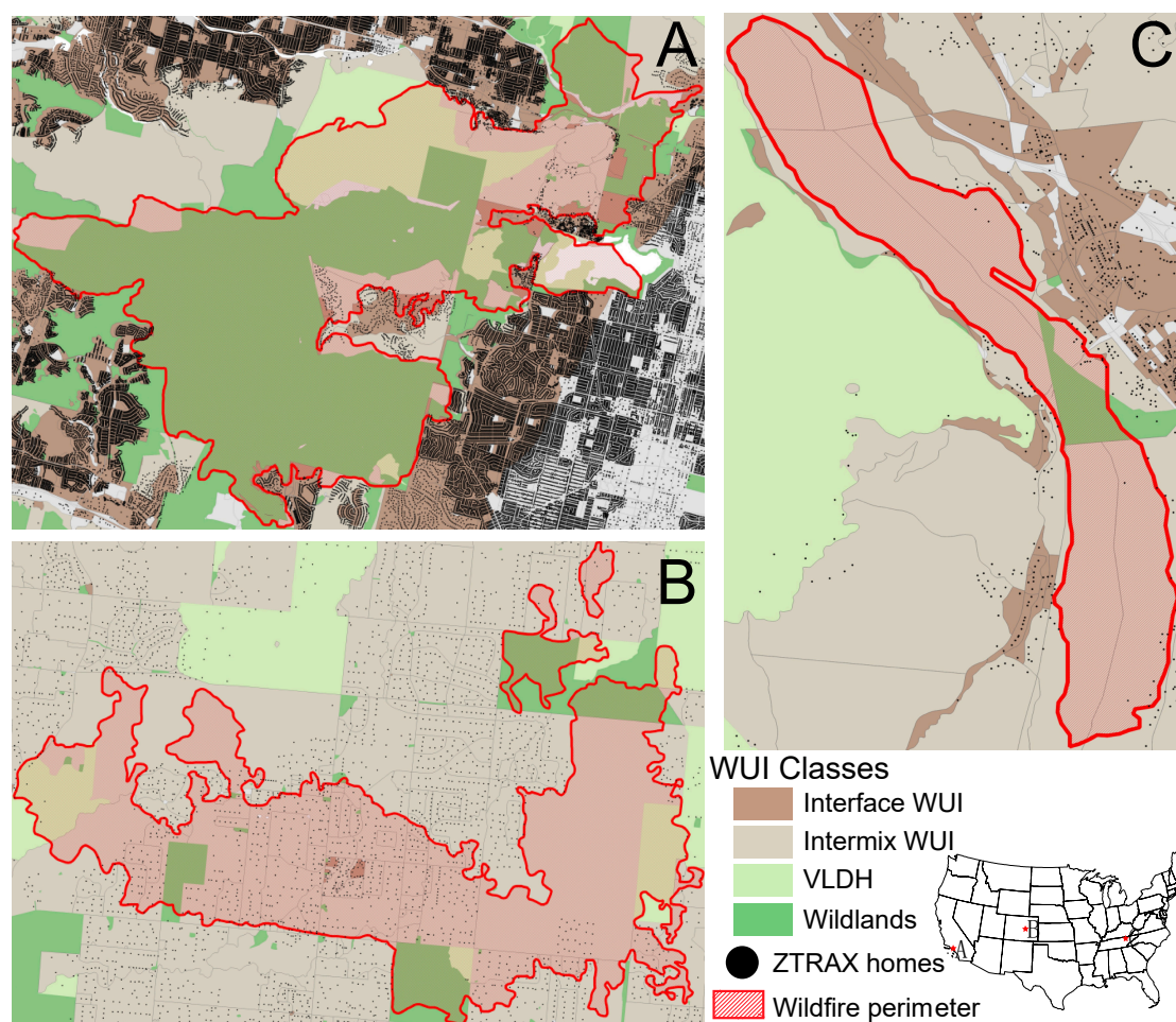
Figure 7. Examples of three wildfires that were human-caused illustrating the enhanced spatial resolution of homes threatened by wildfires using the ZTRAX database compared to the information contained within the census block groups via SILVIS. (A) The Topanga wildfire was an urban, human-caused wildfire near Santa Monica, California that started on 28 September 2005. The WUI dataset estimated 7595 homes, while the ZTRAX estimated 936 homes threatened within the fire perimeter. (B) The Black Forest wildfire was an arson-caused wildfire in the suburbs of Colorado Springs, CO that started on 11 June 2013. The WUI dataset estimated 1480 homes, while the ZTRAX estimated 859 homes threatened within the fire perimeter. (C) A rural, human-caused wildfire from debris burning in northeastern Tennessee that started on 2 March 2006. The WUI dataset estimated 554 homes, while the ZTRAX estimated 54 homes threatened within the fire perimeter.
