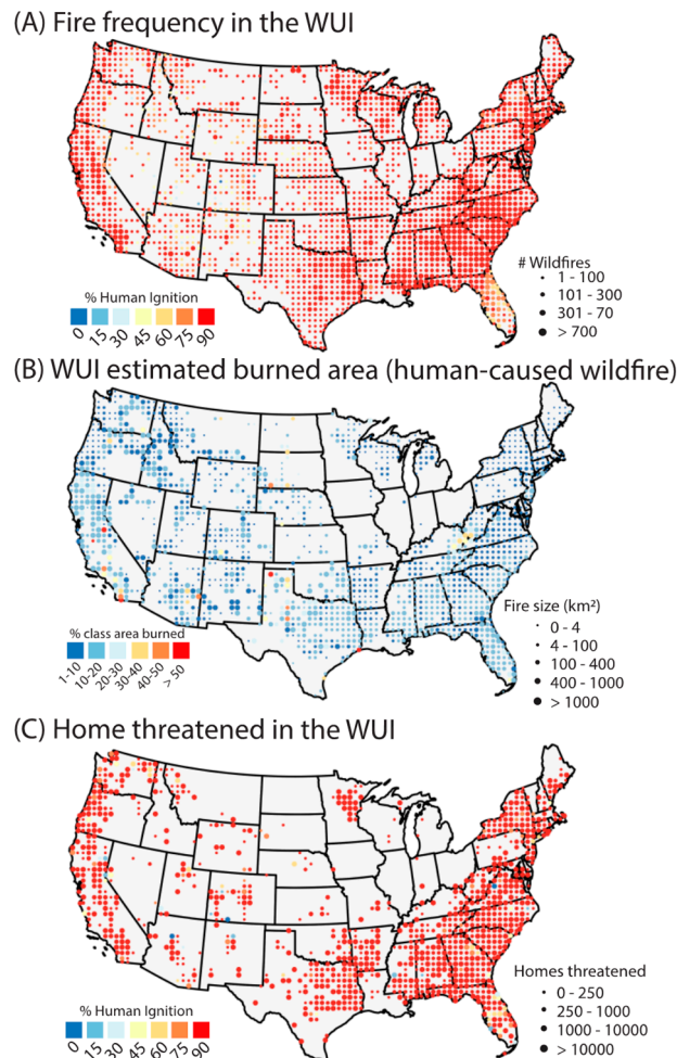
Figure 1. (A) The total number of wildfires (dot size) that originated in the wildland-urban interface stratified by the proportion of wildfires caused by humans, (B) the total fire size (dot size) as a percentage of WUI that was burned by human-caused wildfires, and (C) the total number of homes threatened in the WUI stratified by the proportion of wildfires caused by humans within each 50-km pixel between 1992 and 2015. Black lines represent state boundaries. For (A,C), reds indicate a greater proportion of human-caused wildfires, while blue indicates a greater proportion of lightning-caused wildfires. Note, only the buffer estimated burned area was used (B), not the 250/500/1000 m buffers.
