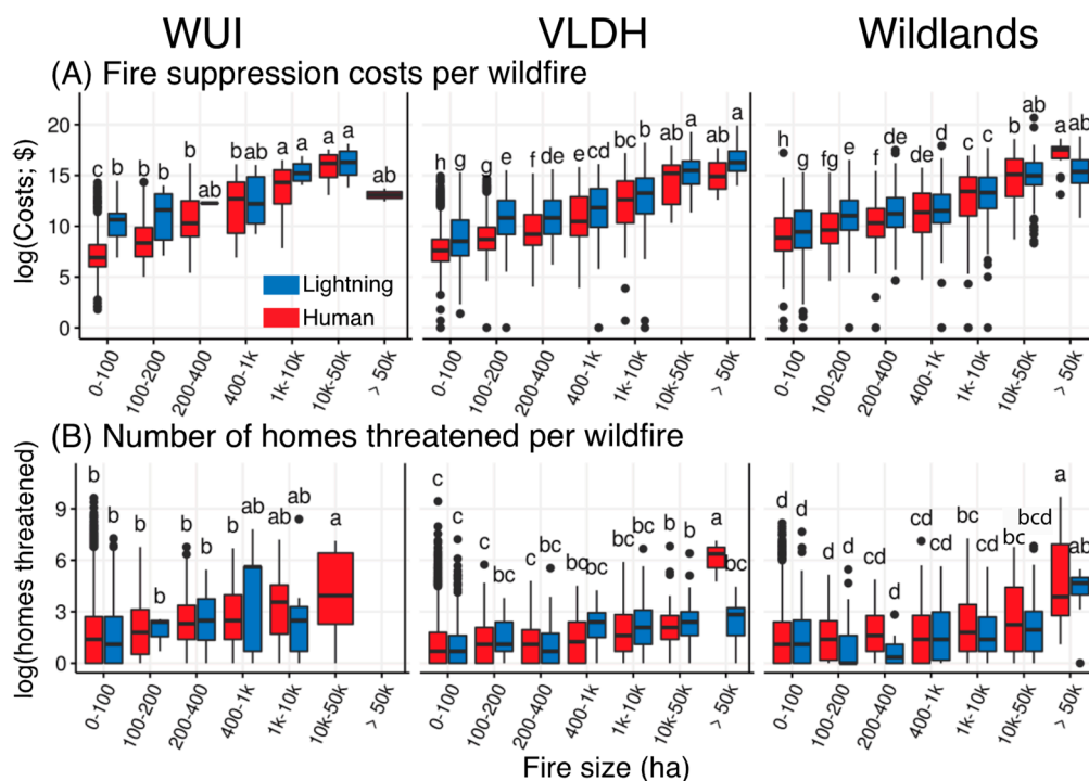
Figure 6. The log mean number of (A) fire suppression costs and (B) homes threatened per human- and lightning-started wildfire event initiated within the wildland-urban interface (WUI), Very low-density housing (VLDH), and wildlands, stratified by fire size in hectares between 1992 and 2015. Error bars indicate the 95th confidence interval around the mean of each group. Tukey's HSD pairwise comparison of the means is represented by differing letters and letter combinations indicating significant differences among groups ( p < 0.0001 ).
