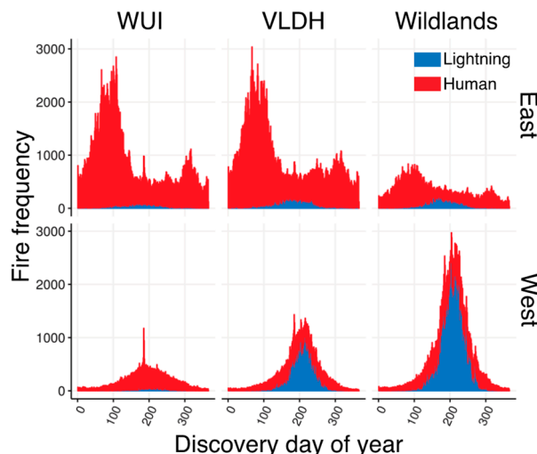
Figure 3. Frequency distributions of human- and lightning-caused wildfires by Julian discovery day of year stratified by wildfires that started either in the wildland-urban interface (WUI), Very low-density housing (VLDH), or wildlands within the eastern or western U.S. between 1992 and 2015.
