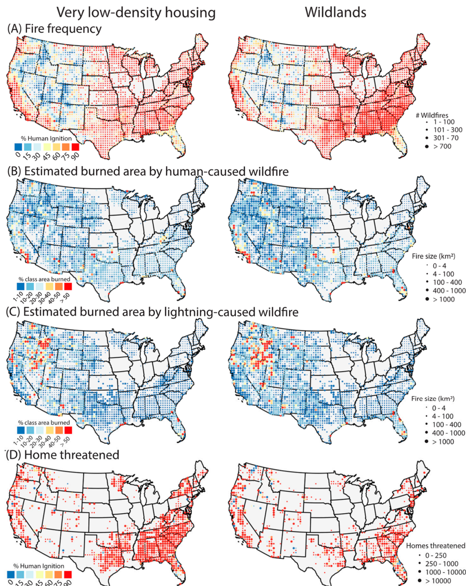
Figure 2. Spatial representation of fire effects in the very-low-density housing and wildlands. (A) The total number of wildfires (dot size) stratified by the proportion of wildfires started by humans, (B) the total fire size (dot size) as a percentage of each class that was estimated burned by human-started wildfires, (C) the total fire size (dot size) as a percentage of each class that was estimated burned by lightning-started wildfires, and (D) the total number of homes threatened stratified by the proportion of wildfires started by humans within each 25-km grid cell from 1992–2015. Black lines represent state boundaries. For (A) and (D), reds indicate a greater proportion of human-started wildfires, while blue indicates a greater proportion of lightning started wildfires.
