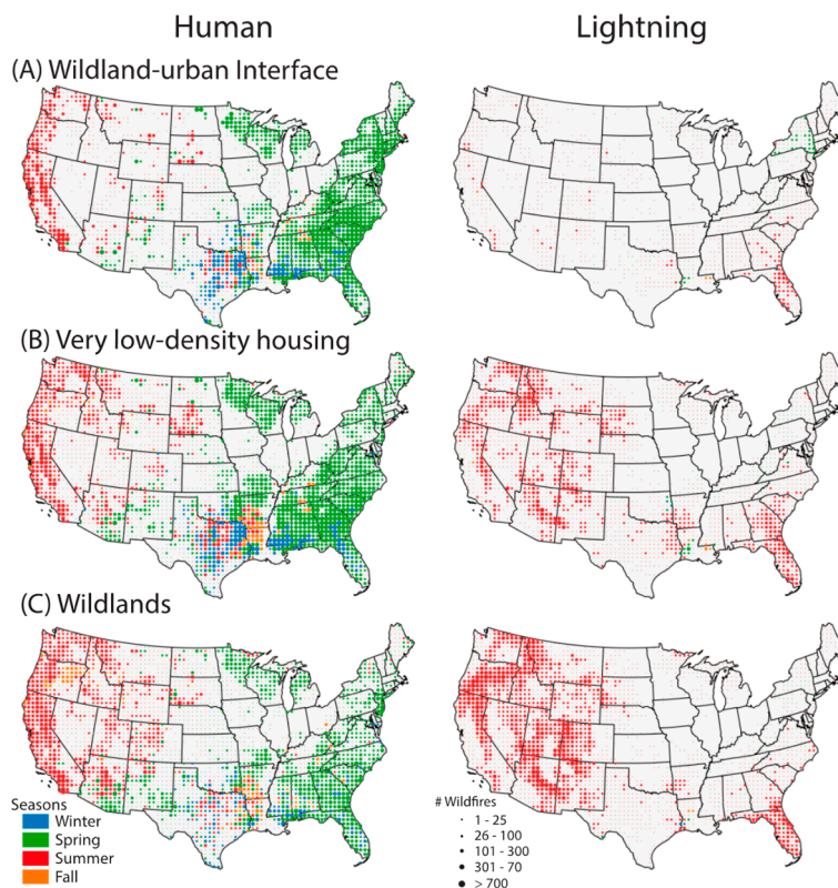
Figure 4. Spatial representation of season that fire ignition was most prevalent across all classes stratified by human and lightning started wildfire in (A) WUI, (B) very-low-density housing, and (C) wildlands. Winter is defined as the months of December, January, February; Spring as March, April, May; Summer as June, July, August; Fall as September, October, December. Dot sizes indicate the total number of wildfire ignitions from 1992–2015 in a 50-km grid cell.
