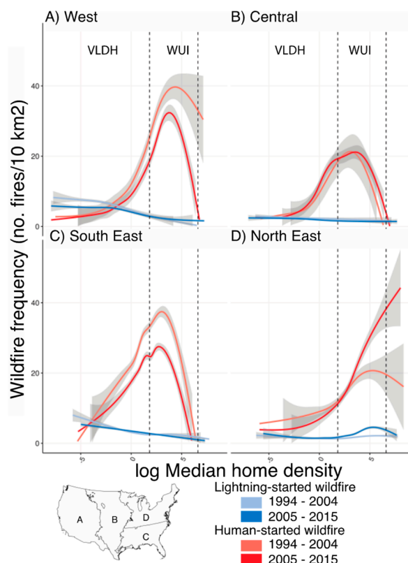
Figure 5. Regional relationships between human- and lightning-caused wildfire ignition frequency and the log median home density within 10-km pixel between two decades (1994–2004 and 2005–2015). Solid lines are based on the best fit Generalized Additive Model regressions with 95th confidence envelope. Dotted vertical lines indicate the division between the WUI and VLDH categories, assuming constant vegetation cover, where urban/WUI boundary equals \log(741.3162) home density and the WUI/VLDH boundary equals \log(6.17) home density.
