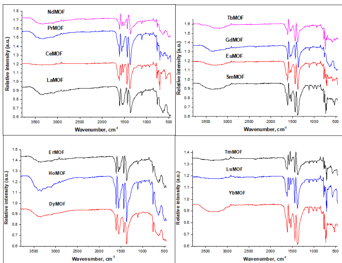
Figure 3. FTIR spectra of LnMOFs.
