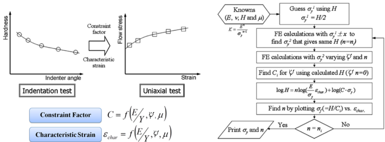
Figure S2: Schematic of the FEA method used based on Shim et al.[41] (right hand side flow chart from Shim et al.[41])
