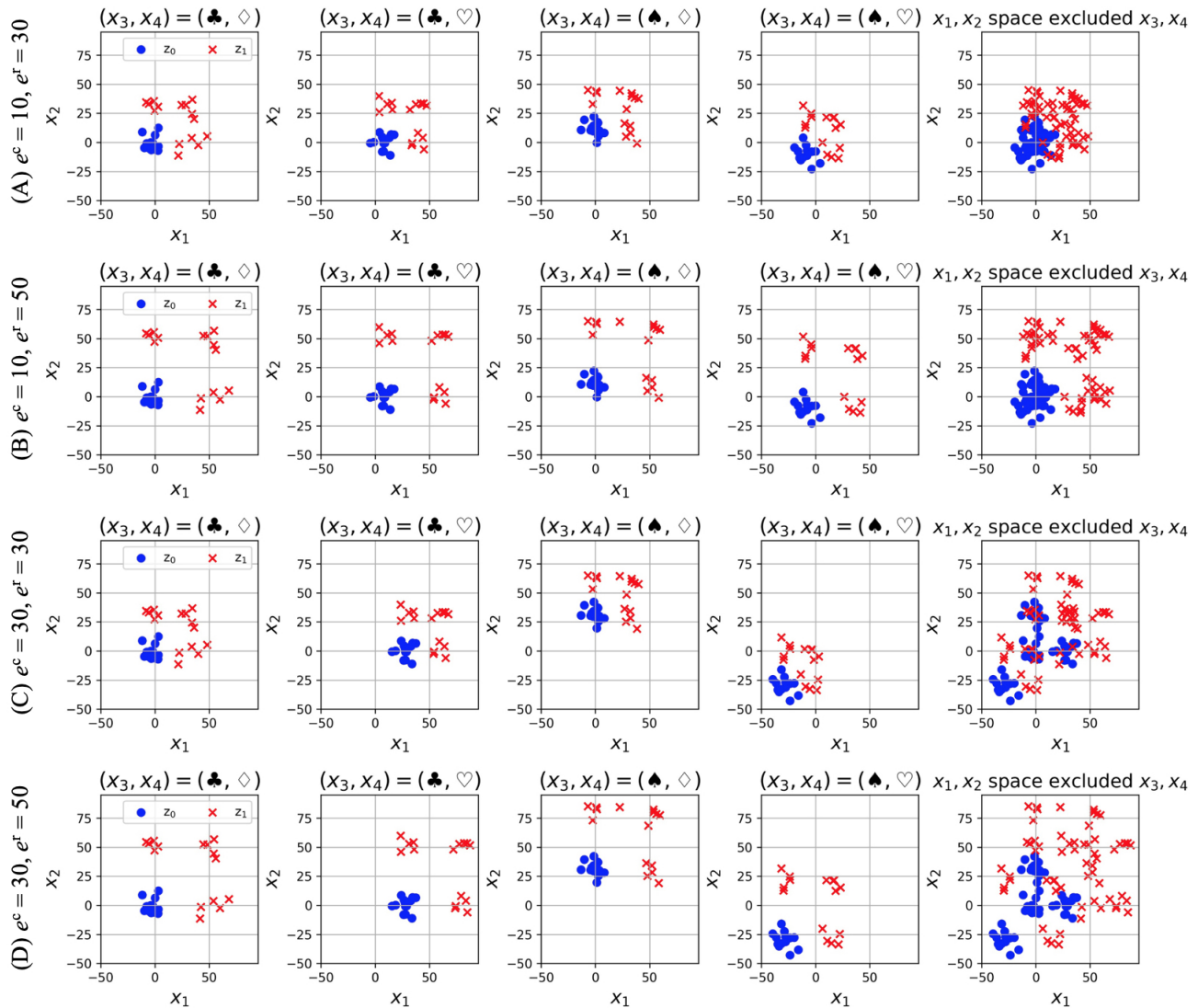
Figure 3. Artificial data generated by using Equations (21) and (23), and Figure 2. The cases (A)–(D) vary in parameters e^c and e^r . The values of categorical features x_3 and x_4 change from left to right. The rightmost figure presents an explicit scatter plot of the numerical features x_1, x_2 , i.e., no categorical features x_3, x_4 are considered.
