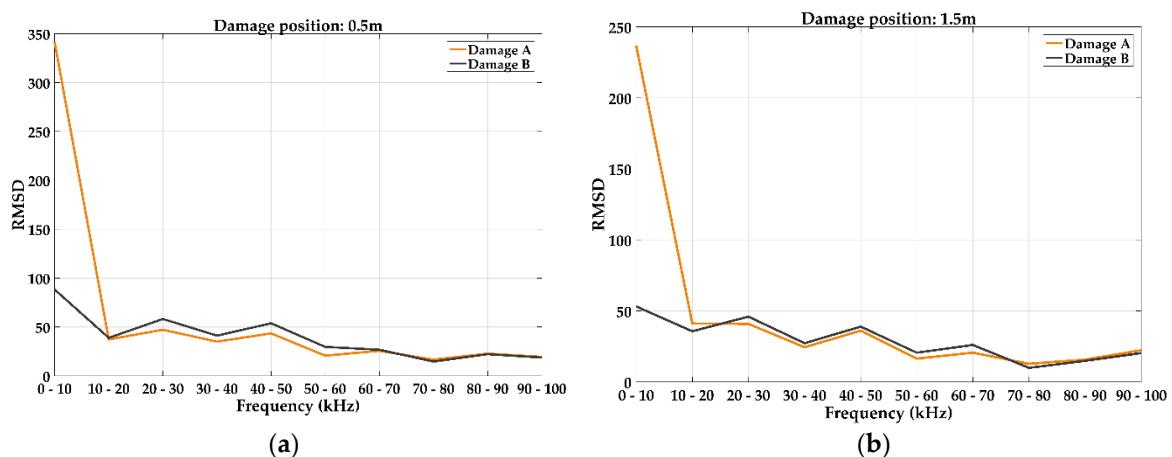
Figure 4. RMSD index for the 0.5 m (a) and 1.5 m (b) positions relative to the transducer.
