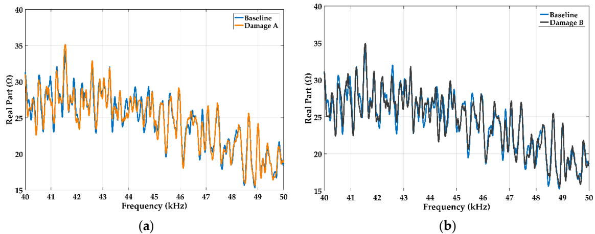
Figure 3. Impedance signatures for damage (a) A and (b) B at 0.5 m from the transducer.
