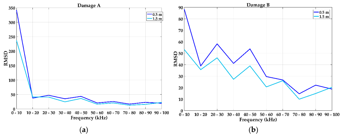
Figure 5. RMSD for damages A (a) and B (b) in two different positions.
