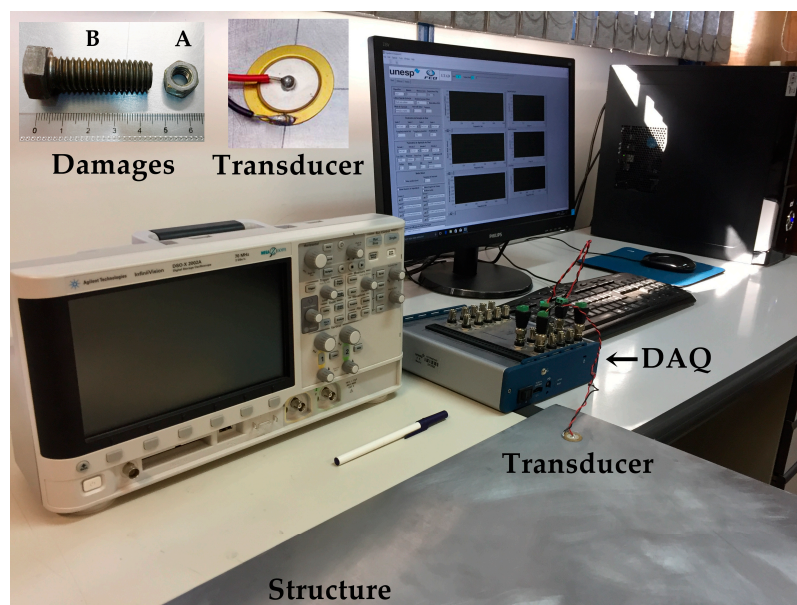
Figure 2. Experimental Setup.
