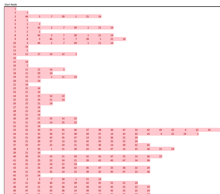
Figure 16. The change propagation path of all start nodes and their members.
