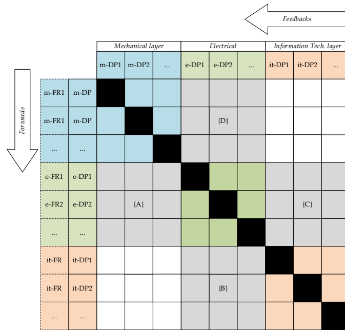
Figure 11. The integration matrix (I-DSM), adapted from [22].
