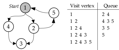
Figure 6. Illustration of breadth-first graph traversal [25].
