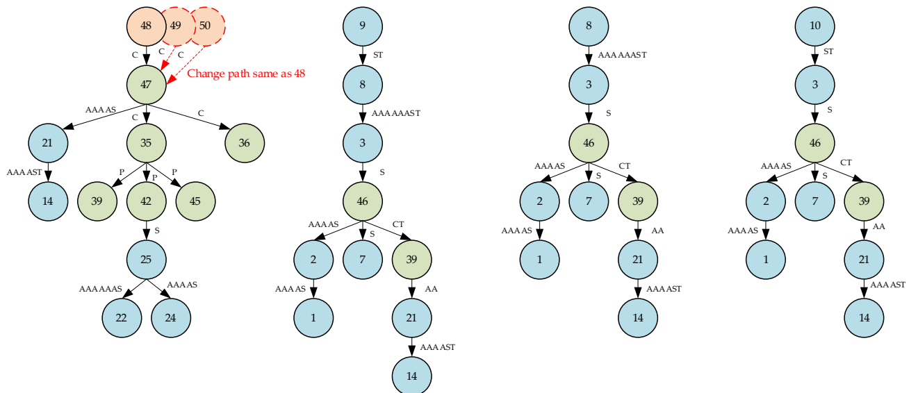
Figure 18. The initial component in other layers of the change propagation path.
