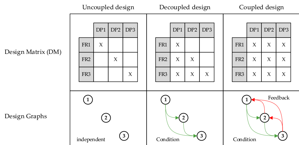
Figure 2. FR–DP relationships according to the design matrix adapted from [1].
