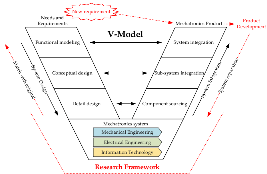
Figure 1. Modeling of mechatronic product investigation.
