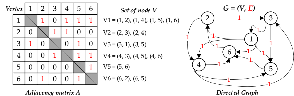
Figure 5. Adjacency matrix A and directed graph G = (V, E) .
