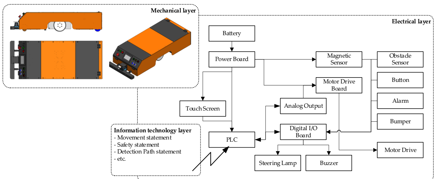
Figure 12. Automatic guided vehicle (AGV) model and mechatronic system.
