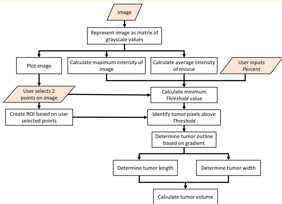
Figure 6. Planar view tumor volume algorithm (PV-TVA) schematic. The user inputs the image and the Percent value, and then selects 2 points on the opposite sides of the tumor. The algorithm then calculates the tumor volume based on the gradient along the line connecting the 2 points that the user selected.
