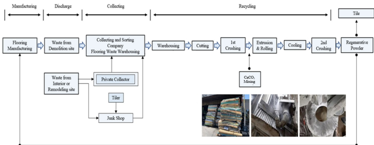
Figure 3. Material flow chart of profile.
