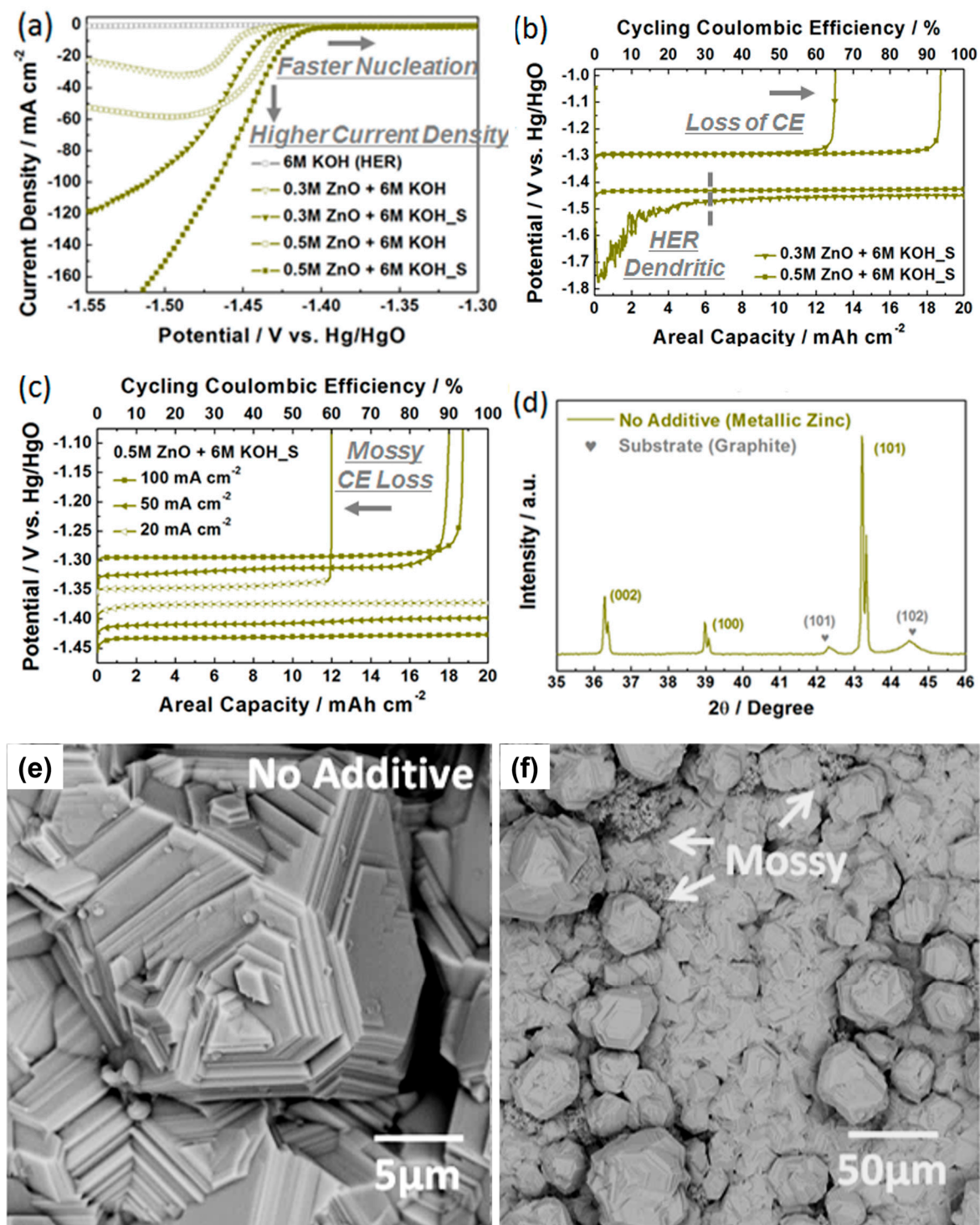
Figure 1. Zinc deposition and dissolution performance of the blank electrolytes without QAAs and the crystallinity/morphology of the zinc deposits derived from no additive. (a) Deposition polarizations for both static and stirred 0.3/0.5 M ZnO + 6 M KOH electrolytes and 6 M KOH only; (b) the 1st zinc deposition–dissolution cycle chronopotentiograms of stirred 0.3/0.5 M ZnO + 6 M KOH at 100 mA cm -2 and 20 mA h cm -2 ; (c) the 1st zinc deposition–dissolution cycle chronopotentiograms of stirred 0.5 M ZnO + 6 M KOH at 20/50/100 mA cm -2 and 20 mA h cm -2 ; (d) XRD pattern between 2θ of 35 to 45° for zinc deposit obtained from no additive, compared with the reference pattern of hexagonal close-packed metallic zinc (JCPDS 03-65-5973); SEM images of zinc deposits obtained from no additive at (e) high (10,000×) and (f) low magnification (1000×). Arrows in (f) point to the mossy structures at boundaries between boulders and base layers.
