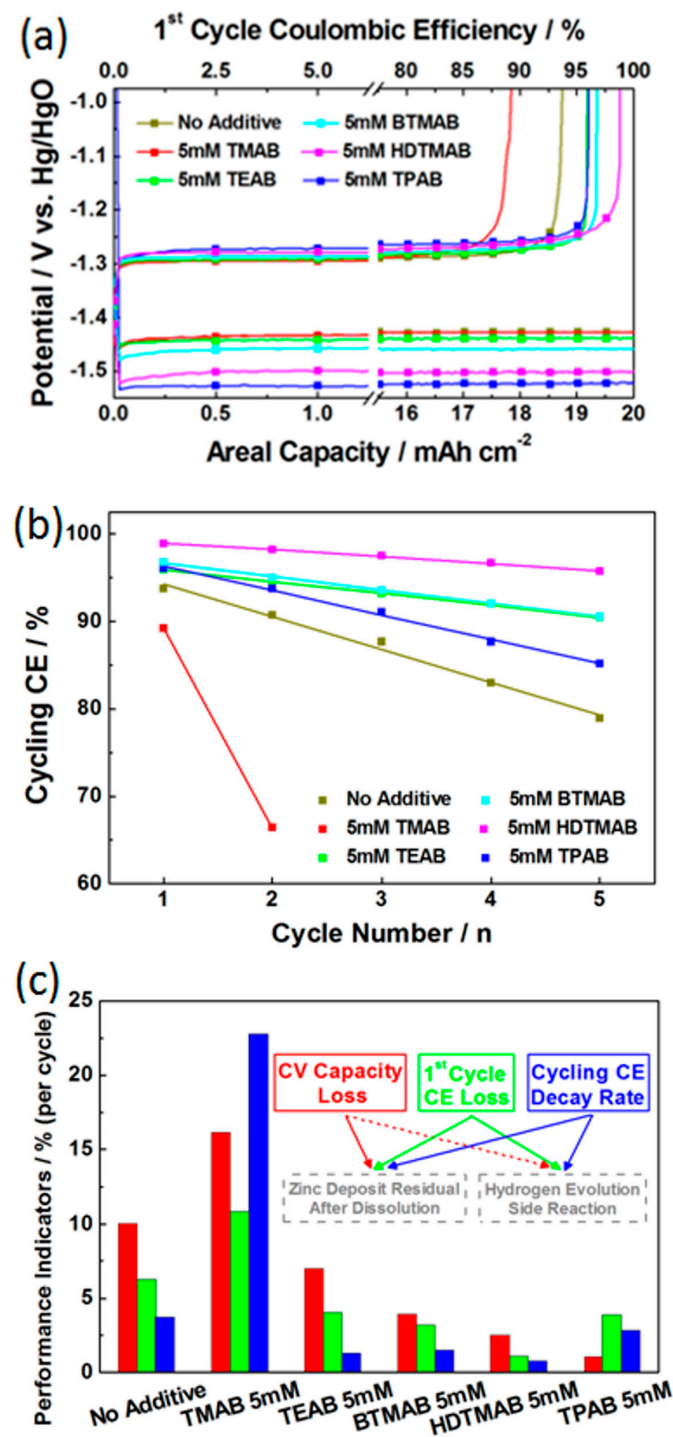
Figure 3. (a) The 1 st zinc deposition–dissolution cycle at 100 mA cm -2 /20 mAh cm -2 , (b) changes of cycling CEs in the 1 st –5 th cycles, and (c) summary of CV charge capacity losses, the 1 st cycle CE losses and cycling CE decay rates for 5 mM TMAB/TEAB/TPAB/BTMAB/HDTMAB and no additive. The values of areal capacity and coulombic efficiency in (a) are directly calculated based on charge/discharge time.
