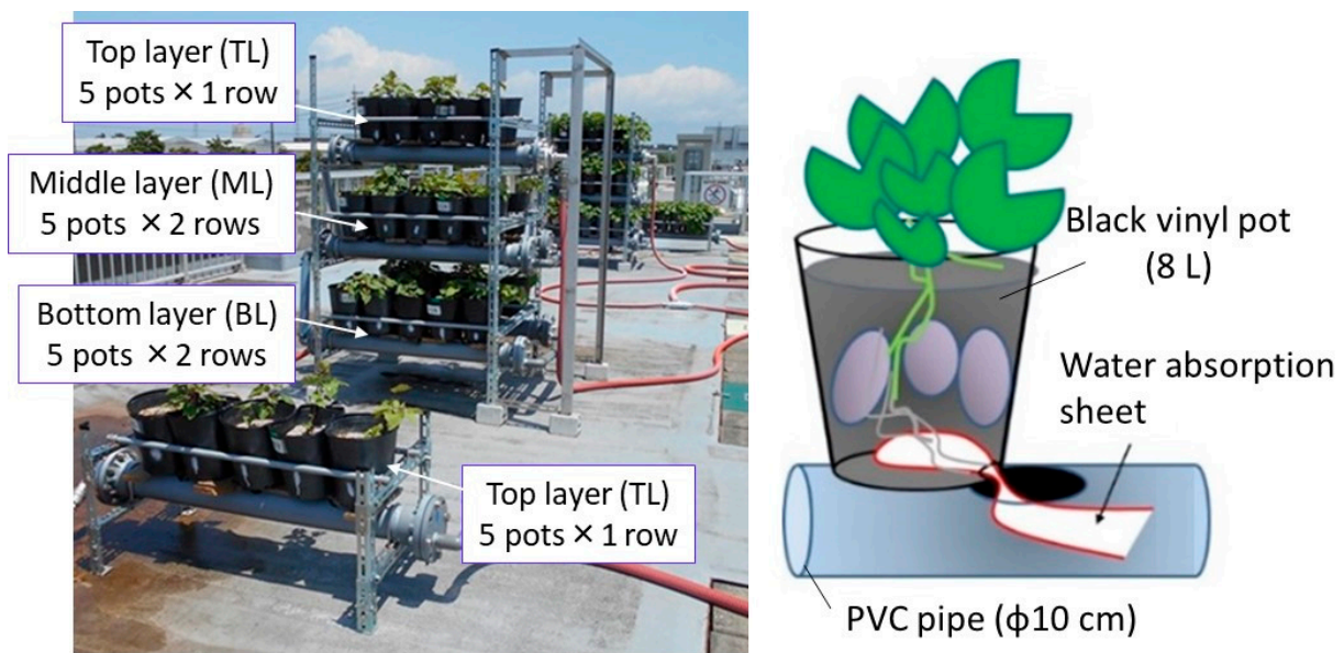
Figure 2. The three-layer cultivation system with rhizosphere irrigation.
