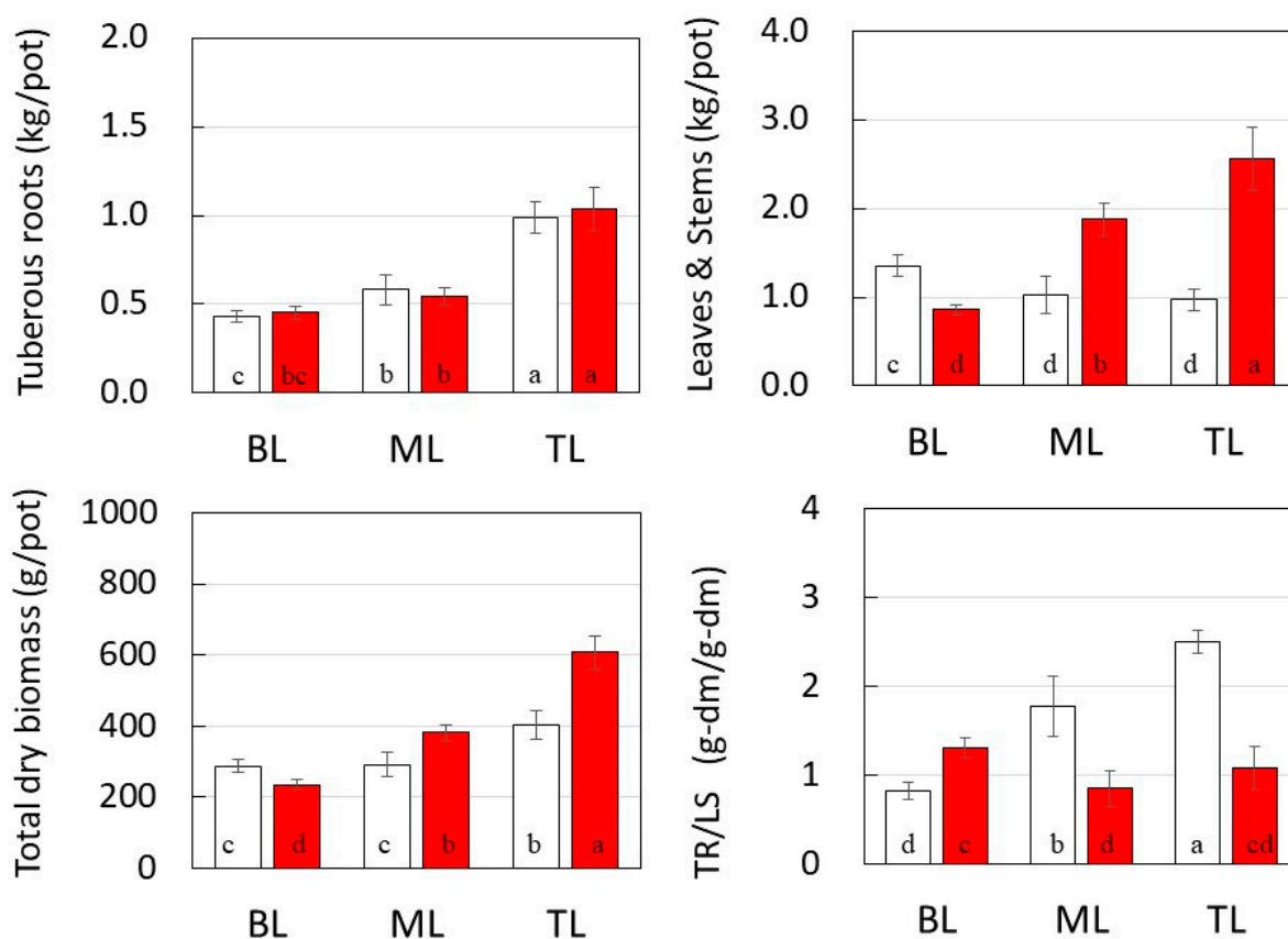
Figure 9. The fresh weight of tuberous roots, leaves and stems, the total dry biomass weight and the dry weight ratio of tuberous roots (TR) to leaves and stems (LS) per pot harvested in bottom layer (BL), middle layer (ML) and top layer (TL). Symbols: □, SK; ■, BH. Data are means and error bars represent standard error of the mean. Different letters indicate statistically significant differences between cultivation layers ( p < 0.05 ).
