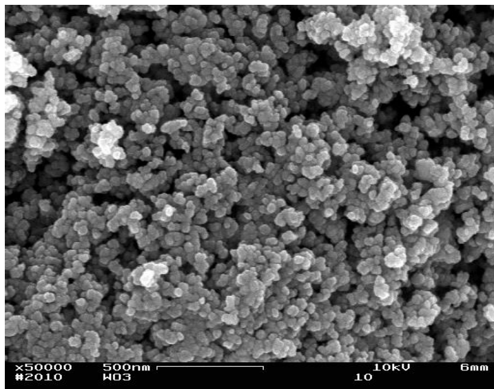
Figure 2. SEM view of the pristine \text{WO}_3 material.
