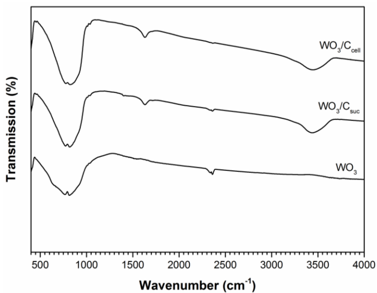
Figure 1. FTIR spectra of the different \text{WO}_3/\text{C} composites. The pristine \text{WO}_3 material is also reported.
