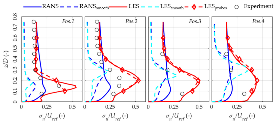
Figure 9. Longitudinal turbulence intensity for positions 1–4. The continuous line refers to the turbulent inlet, and the dashed line to the smooth inlet. LES results were computed using both ensemble averages and time averages from probes for comparison.
