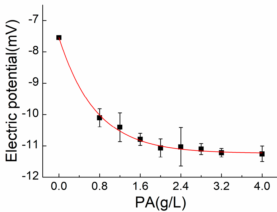
Figure S2. The \zeta -potential of the PA-OSH complex as a function of the PA concentration. The OSH concentration is 1 g/L for all samples.
