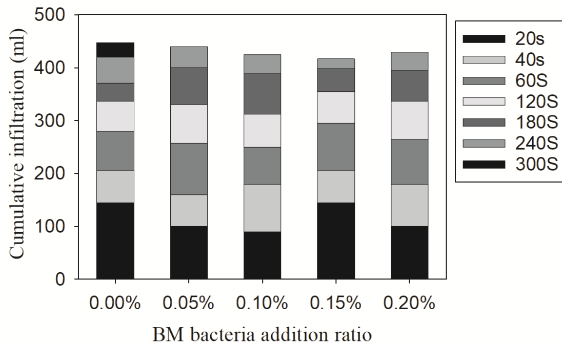
Figure.S2 Variation characteristics of cumulative infiltration of complex soil with different BM addition ratio within 5 min. The percentage represents BM added mass ratio.
