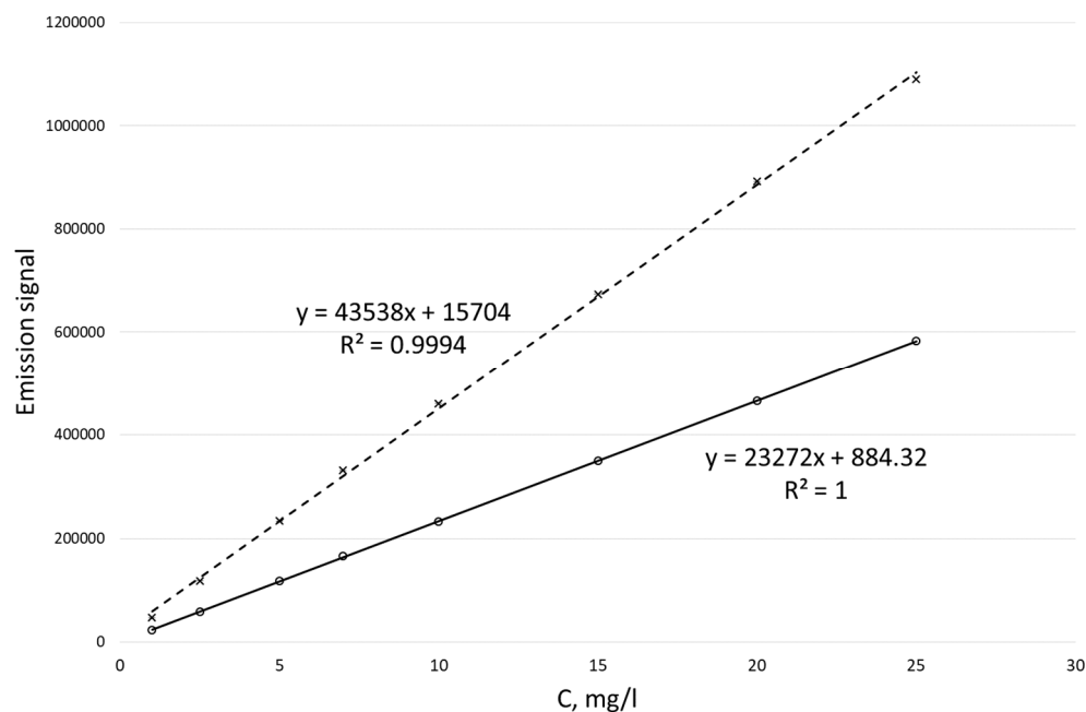
Figure 2. Calibration curves for the determination of potassium ion concentration by the MIP-OES method for two wavelengths at 766.49 nm (dotted line) and 769.89 nm (solid line).
