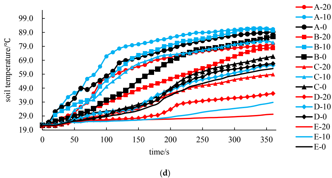
Figure 12. Variation diagram of ST and disinfection time in each layer: (a) <2 mm; (b) 7–17 mm; (c) 17–27 mm; (d) >27 mm. Note: A-20 indicates that A is the test point, and 20 is the test depth (–20 cm). The same conditions apply in the following section.
