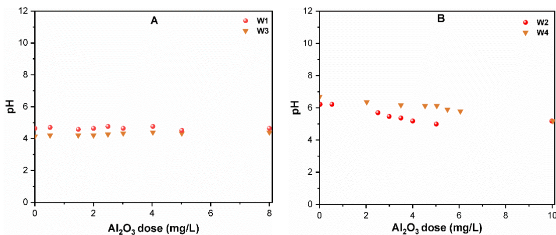
Figure. S1. Difference of water pH with added coagulant for: (A) hydrophilic; (B) hydrophobic waters
