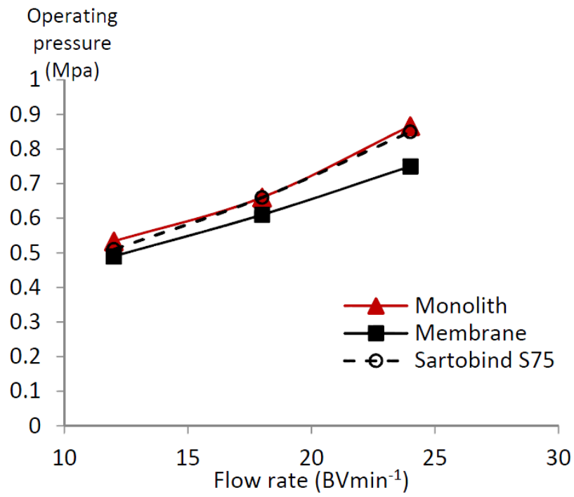
Supplementary data 1. Average operating pressures during the BSA-LF mixture loading step at flow rates of 12.0, 18.0 and 24.0 BV·min -1 using the monolith ( H = 3 mm), membrane ( H = 3 mm) in the CIM housing and Sartobind S75 device ( H = 4 mm).
