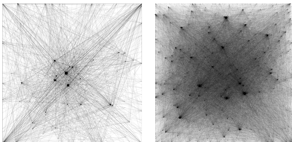
Figure 2. Visual representation of the LN. The plot on the left refers to 2018/02/12, while the one on the right to 2020/08/12.
