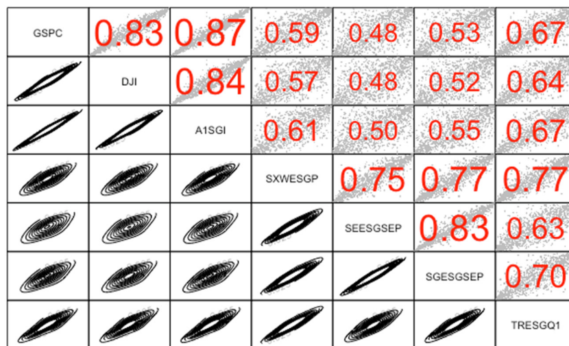
Figure 4. Kendall's \tau and copulas, 2 December 2009–30 July 2014.
