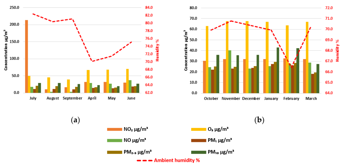
Figure 5. Mean humidity, and concentration values of air pollutants ( \text{NO}_2 , \text{O}_3 , \text{NO} , \text{PM}_{10} , \text{PM}_{2.5} ) during the rainy (July to September 2020, April to June 2021) and dry (October 2020 to March 2021) seasons. (a) Rainy season. (b) Dry season.
