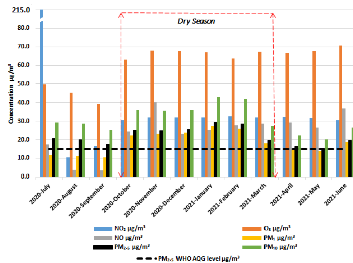
Figure 6. Concentration values of air pollutants ( \text{NO}_2 , \text{O}_3 , \text{NO} , \text{PM}_1 , \text{PM}_{2.5} , \text{PM}_{10} ) during the rainy (July to September 2020, April to June 2021) and dry (October 2020 to March 2021) seasons, with the recommended 24 h average \text{PM}_{2.5} WHO Air Quality Guidelines concentration level.
