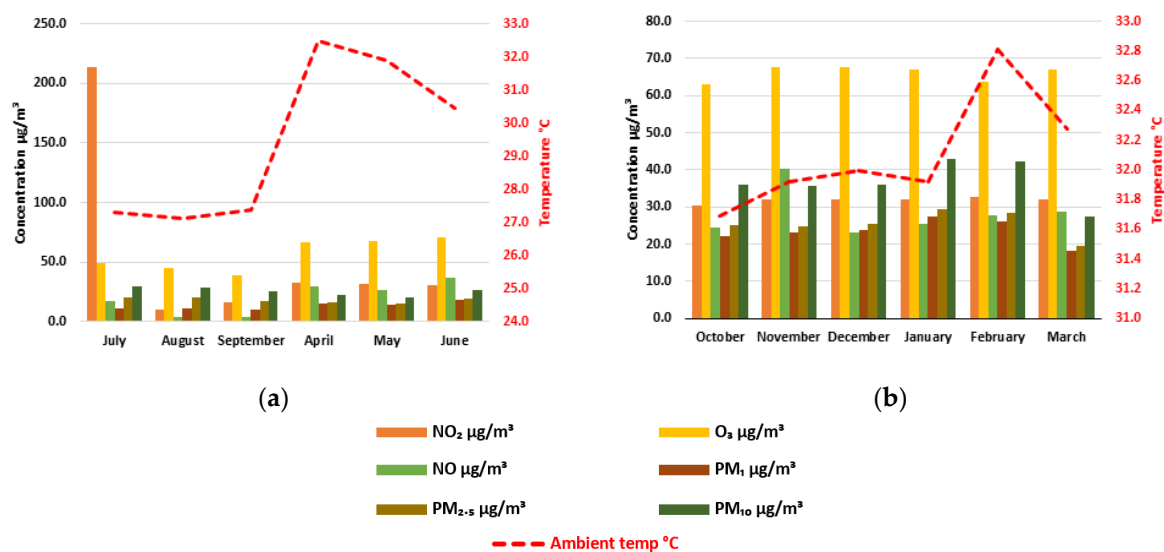
Figure 4. Mean temperature, and concentration values of air pollutants ( \text{NO}_2 , \text{O}_3 , \text{NO} , \text{PM}_{10} , \text{PM}_{2.5} ) during the rainy (July to September 2020, April to June 2021) and dry (October 2020 to March 2021) seasons. (a) Rainy season. (b) Dry season.
