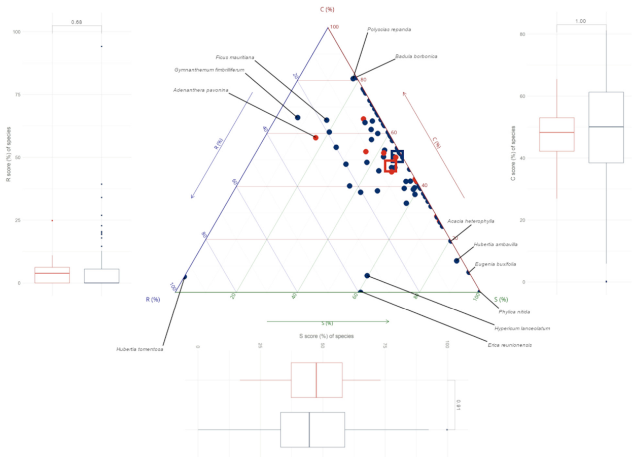
Figure 6. Comparison between the ecological strategies of native and alien tree species sampled in Saint-Philippe (Réunion). The three-dimensional diagram shows the CSR scores of native (blue circles, n = 70 ) and alien species (red circles, n = 10 ) and their respective median (blue and red squares, respectively). The C (red), S (green), and R (blue) axes represent the competitiveness, stress tolerance, and ruderalism of each species, respectively. The boxplots compare of the CSR scores obtained for native (blue, n = 67 , i.e., without tree ferns) and alien species (red, n = 10 ). p -values of ANOVA accounting for the phylogeny in which the R scores were log-transformed are indicated.
