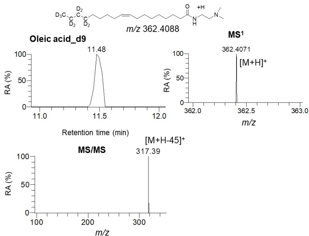
Figure S1: Extracted ion chromatogram and mass spectra of internal standard oleic acid-d9
