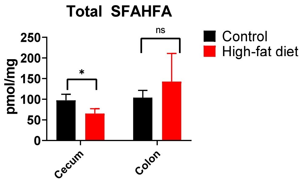
Figure S3: Total SFAHFAs comparison between colon and cecum contents.
