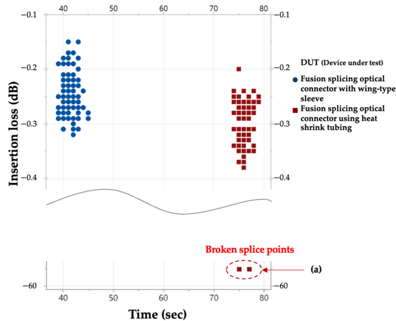
Figure 21. Comparison of splice loss and splice time of two types of DUTs.
