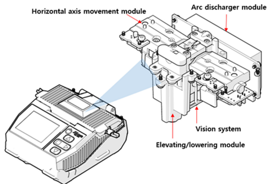
Figure 8. Internal structure of the developed fusion splicer for fusion splicing of optical connectors.
