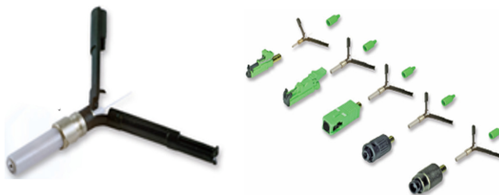
Figure 4. A fusion-spliced optical connector head with a wing sleeve.
