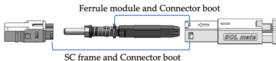
Figure 6. Cable boot mounting structure in our design.
