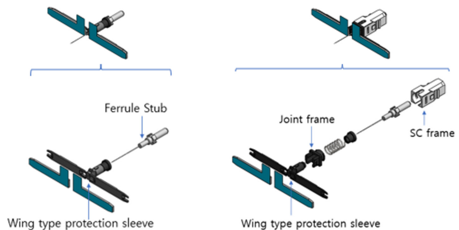
(a) Structure of an existing product
