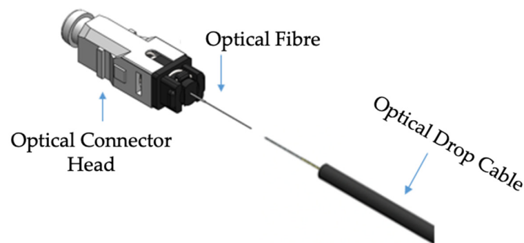
Figure 2. Fusion splicing of an optical connector head.
