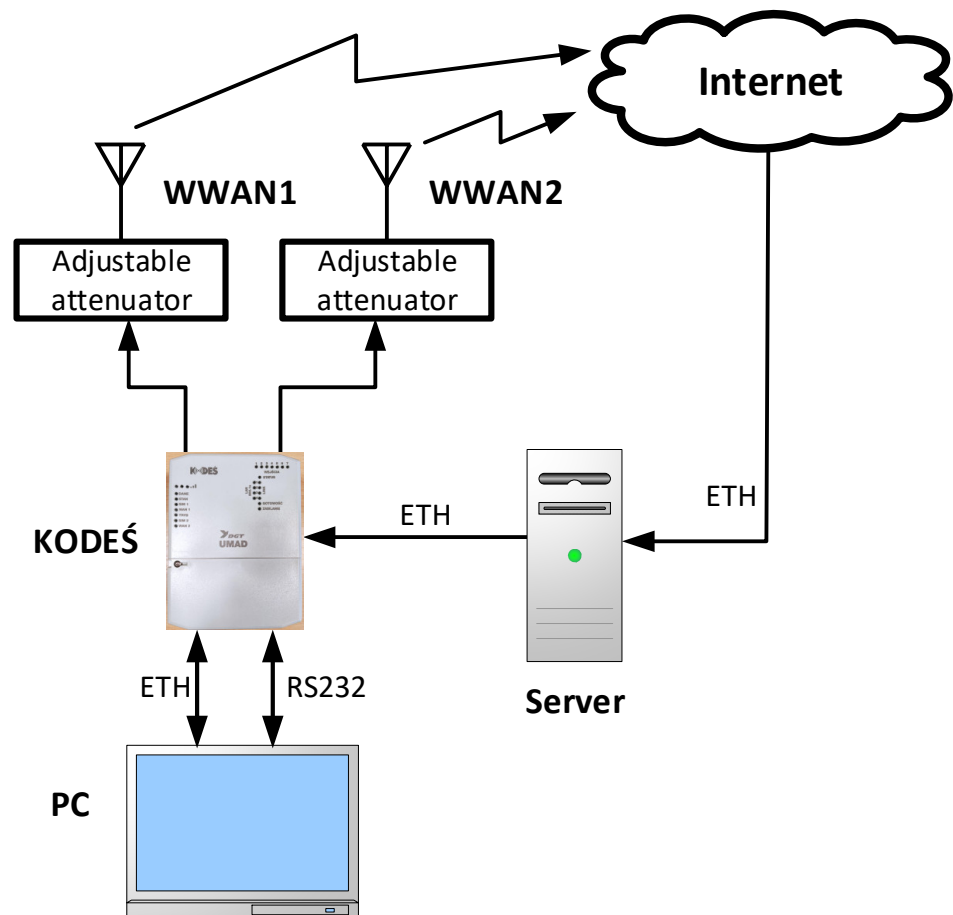
Figure 3. Laboratory stand.
