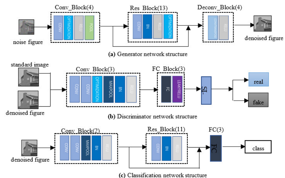
Figure 3. Sub-network structures.
