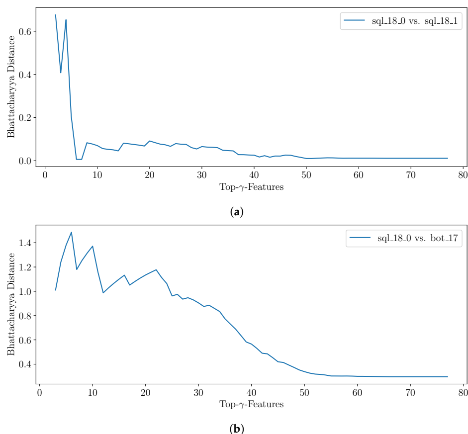
Figure 10. The dependency of \gamma on the Bhattacharyya distance (similarity) of two highly similar (a) and dissimilar (b) attack scenarios.
