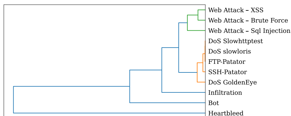
Figure 8. Hierarchical clustering of similarities between CICIDS2017 attack scenarios based on sig_{com} .
