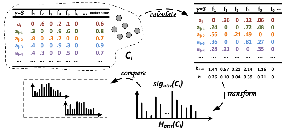
Figure 5. The generation and comparison process of the signature sig_{attr} .
