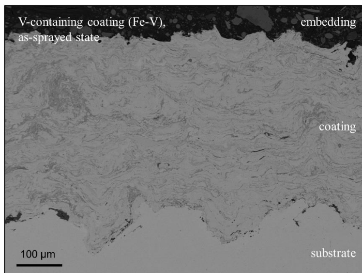
Figure S1. SEM image showing the cross section of the produced V-containing Fe-based coating.
